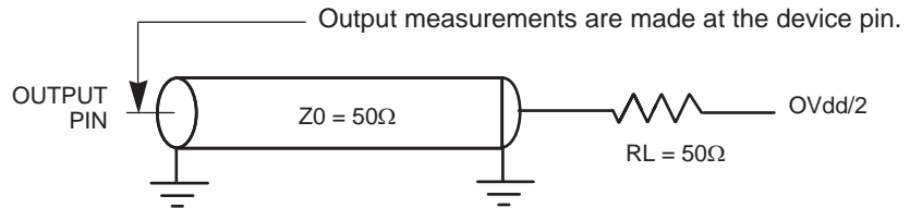
Figure 13. AC Test Load for the PC107A
