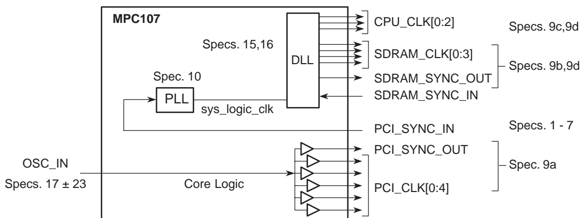
Figure 8. Clock Subsystem Block Diagram
