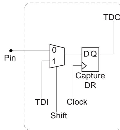
Pin BSC
