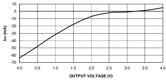
OUTPUT SOURCE CURRENT VS. OUTPUT VOLTAGE ( V_{CC} = 3.3V , T_A = 25^\circ C )
