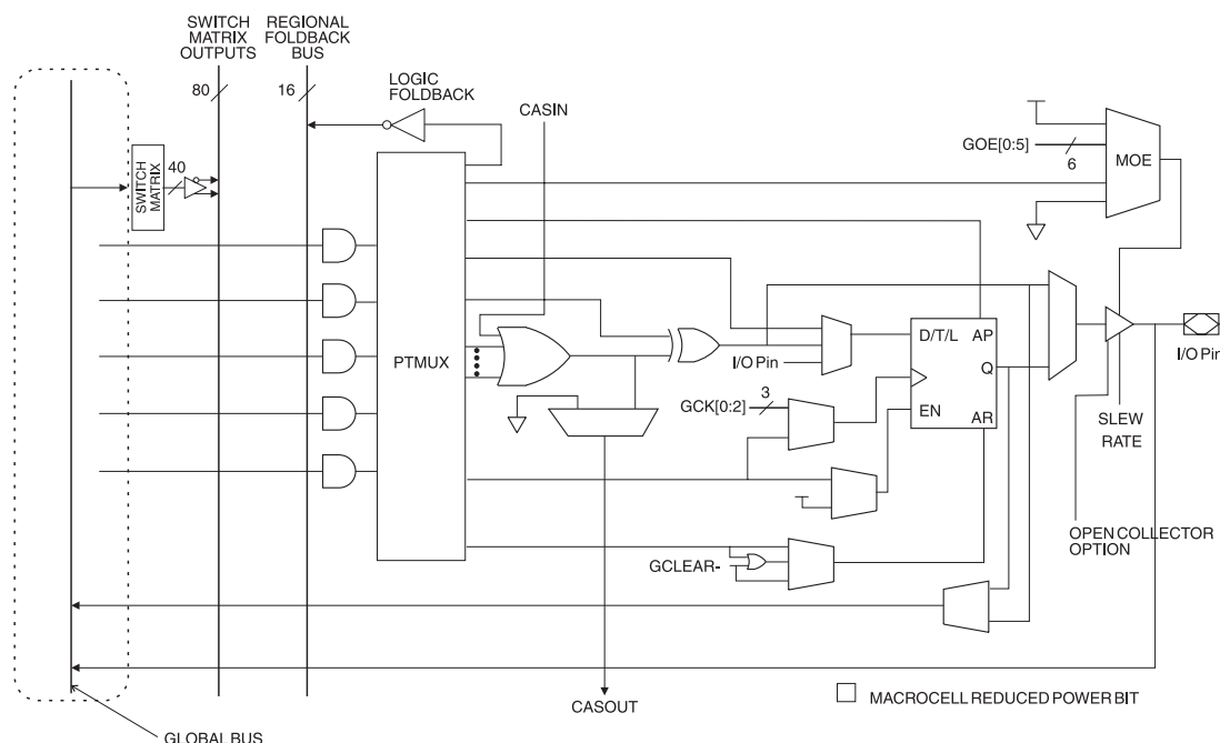
Figure 1. ATF1502AS Macrocell
