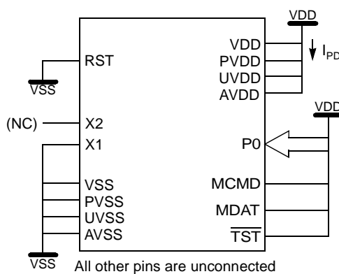
Figure 141. I_{PD} Test Condition, Power-Down Mode
