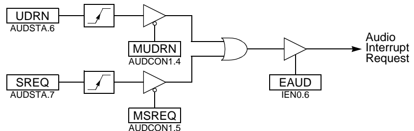
Figure 54. Audio Interface Interrupt System
