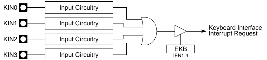
Figure 137. Keyboard Interface Block Diagram
