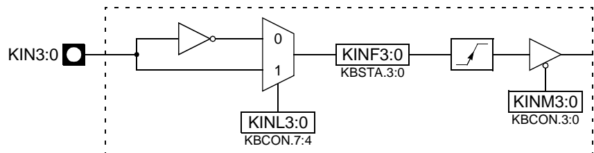
Figure 138. Keyboard Input Circuitry
