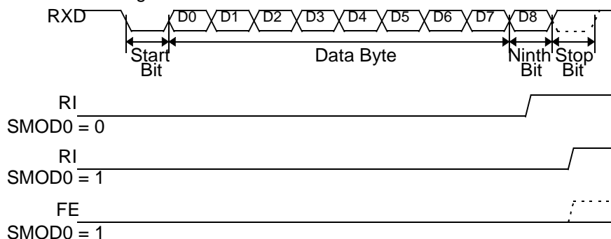
Figure 3. UART Timings in Modes 2 and 3
