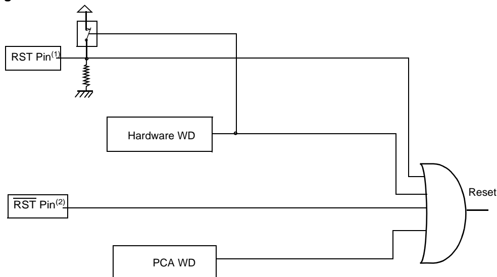
Figure 1. Reset Sources
