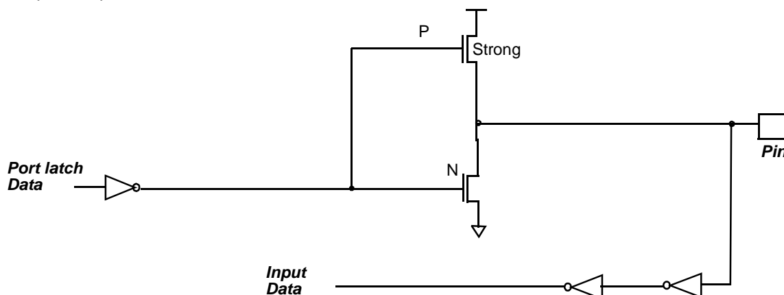
Figure 3. Push-pull Output
