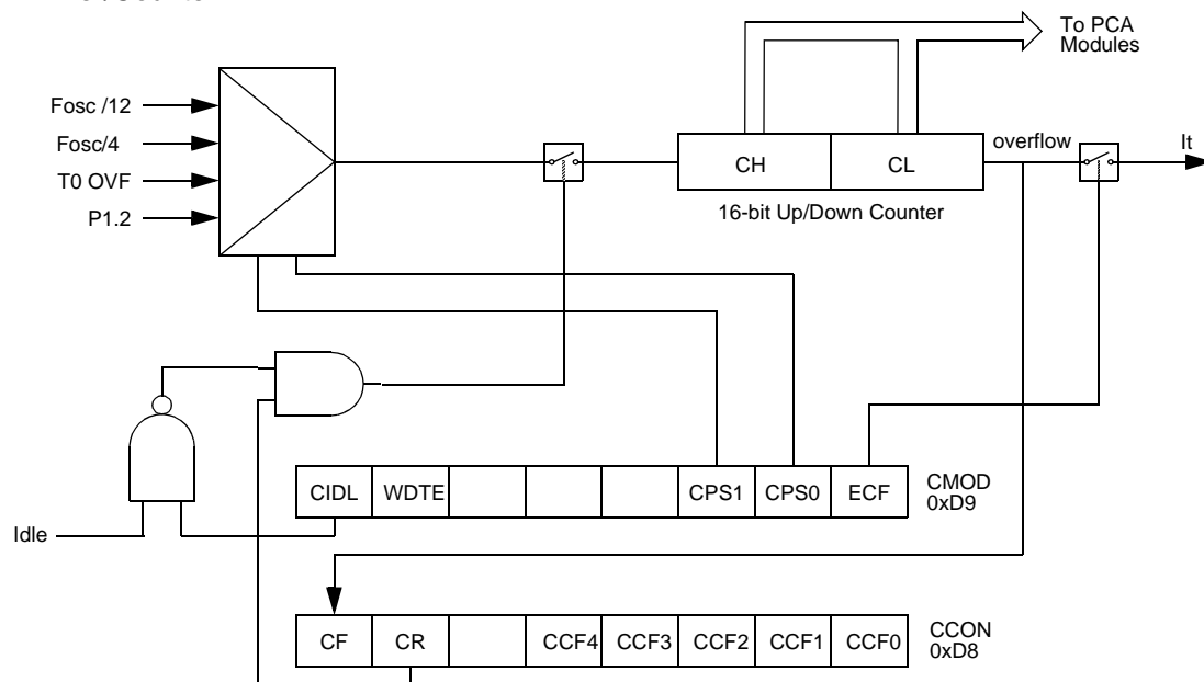
Figure 1. PCA Timer/Counter
