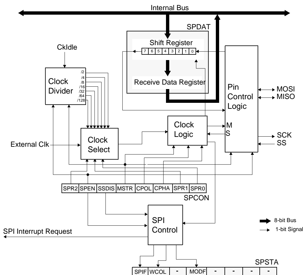
Figure 2. SPI Module Block Diagram
