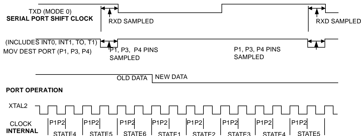
Figure 10. Clock Waveforms
