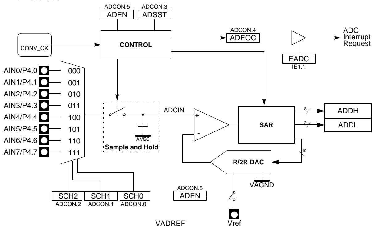
Figure 1. ADC Description
