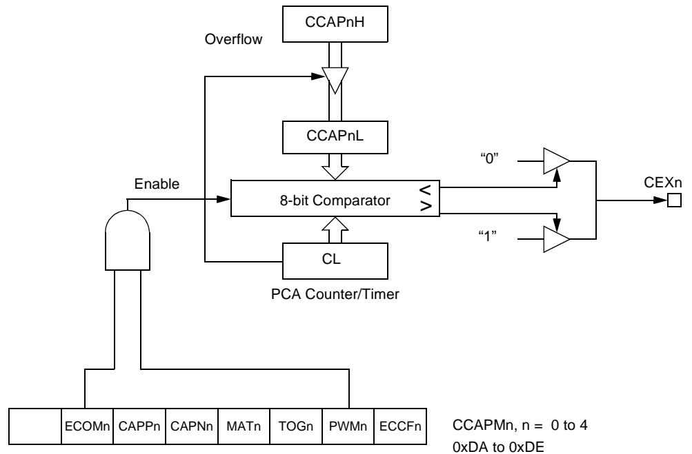
Figure 6. PCA PWM Mode
