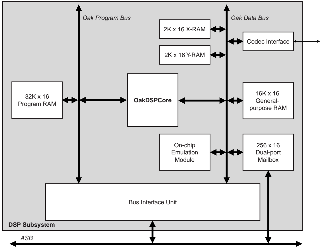
Figure 4. DSP Subsystem
