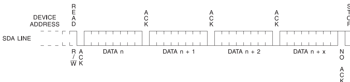
Figure 12. Sequential Read
