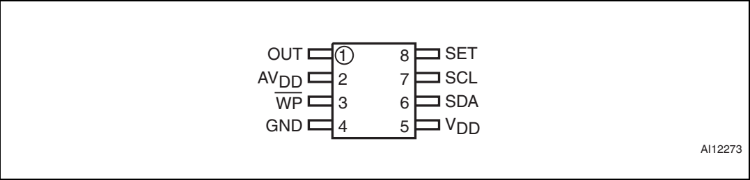
Figure 2. Connections diagram
