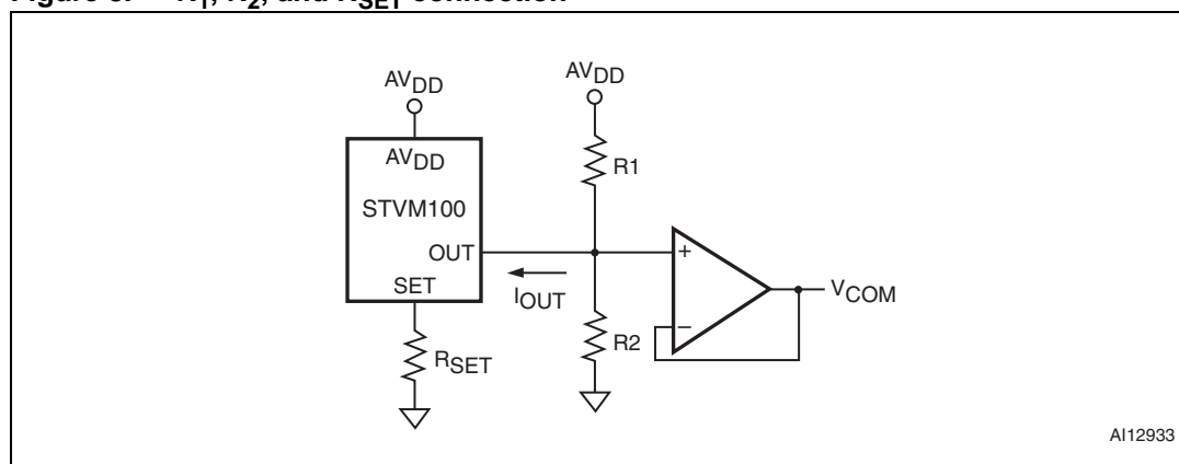
Figure 8. R_1 , R_2 , and R_{SET} connection
