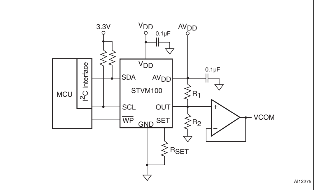
Figure 4. Hardware hookup
