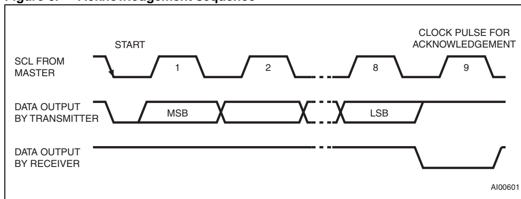
Figure 6. Acknowledgement sequence
