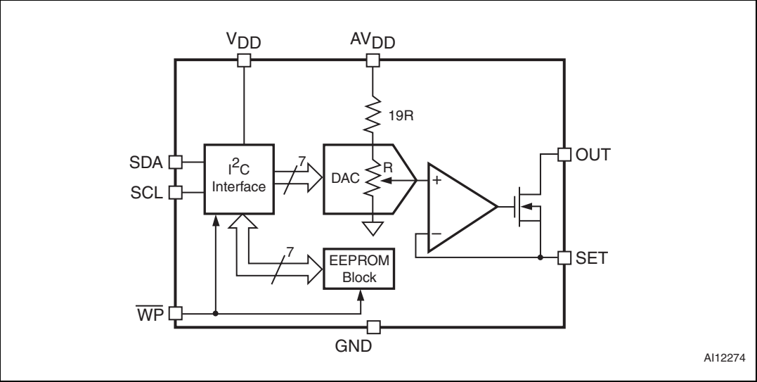
Figure 3. Block diagram
