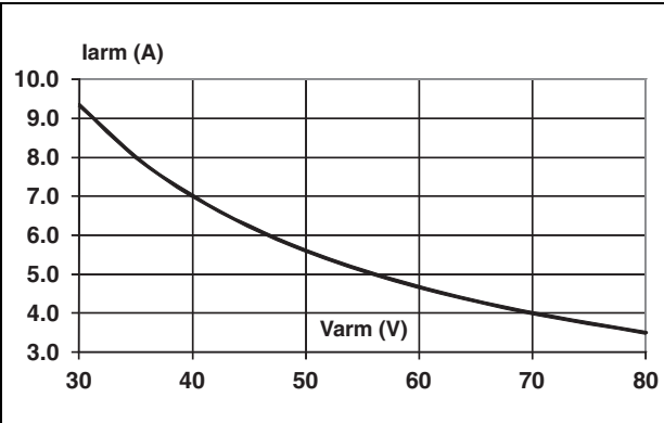
Figure 8. Reverse safe operating area ( t_p < 10 \mu s and T_j < 125^\circ C )
