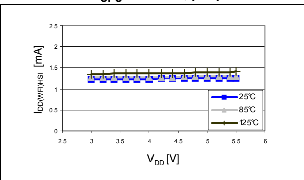
Figure 15. Typ. I_{DD(WFI)HSE} vs. V_{DD} @ f_{CPU} = 16 MHz, peripheral = off
