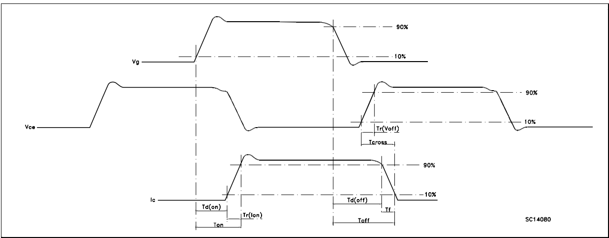
Fig. 3: Switching Waveforms
