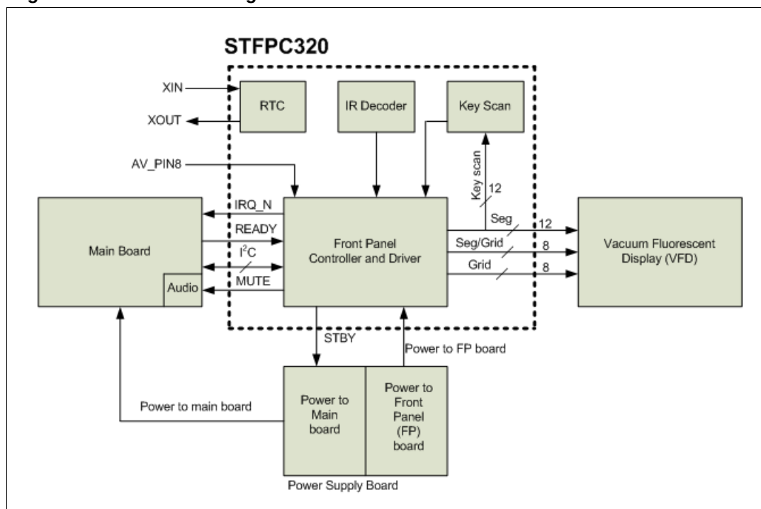
Figure 2. Functional diagram
