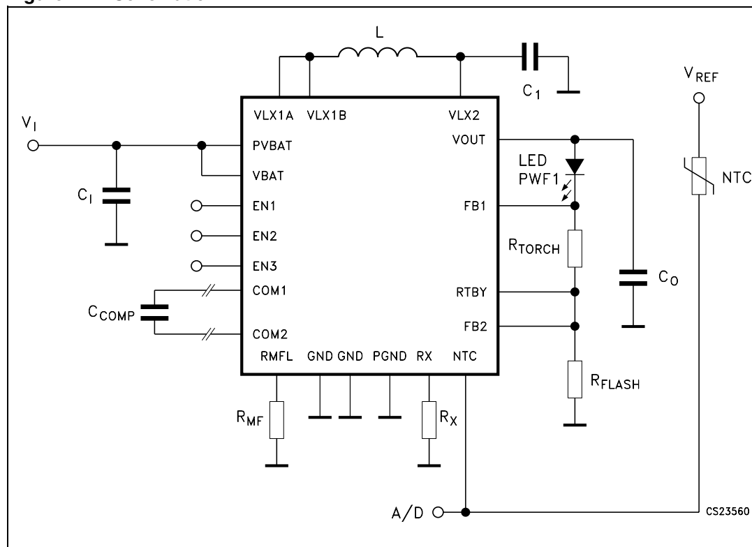
Figure 1. Schematic
