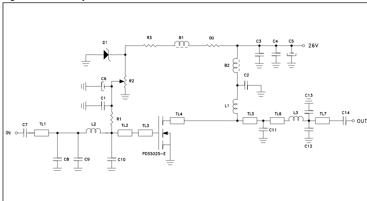
Figure 2. Circuit layout
