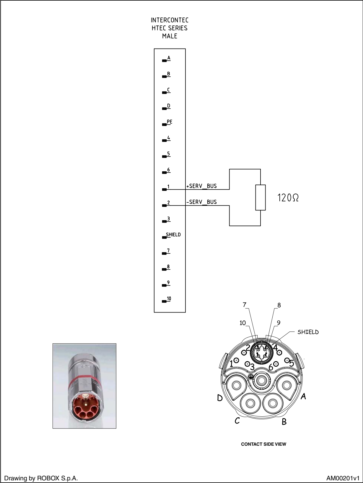
Figure 6. CAVO1SPIMD terminal
