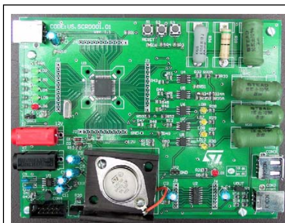
STEVAL-PCN001V1
