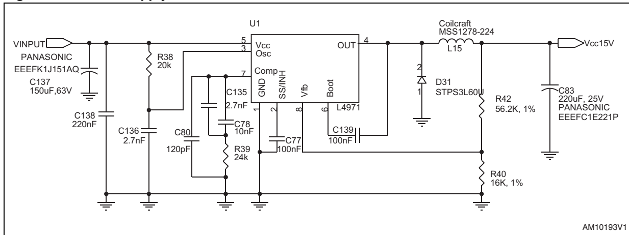
Figure 3. Power supply section - 5 V
