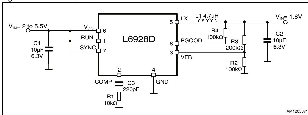
Figure 1. Circuit schematic
