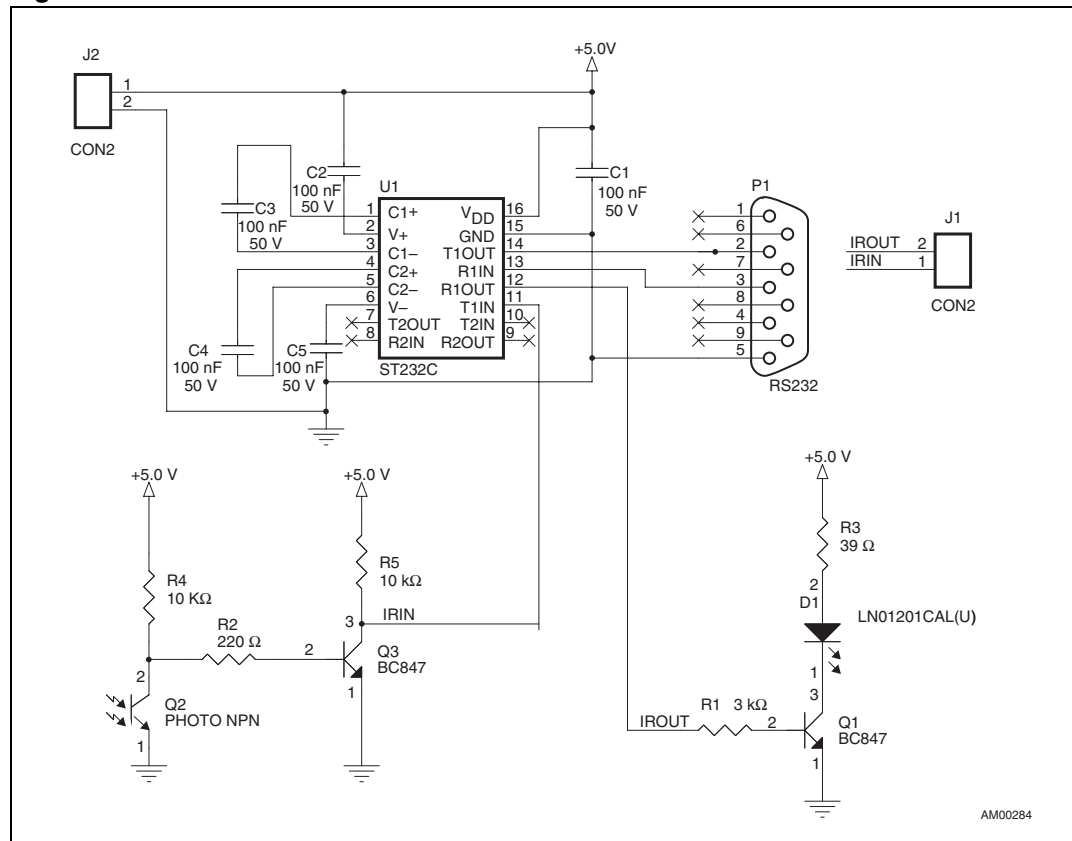
Figure 4. Schematic - SCI-interface
