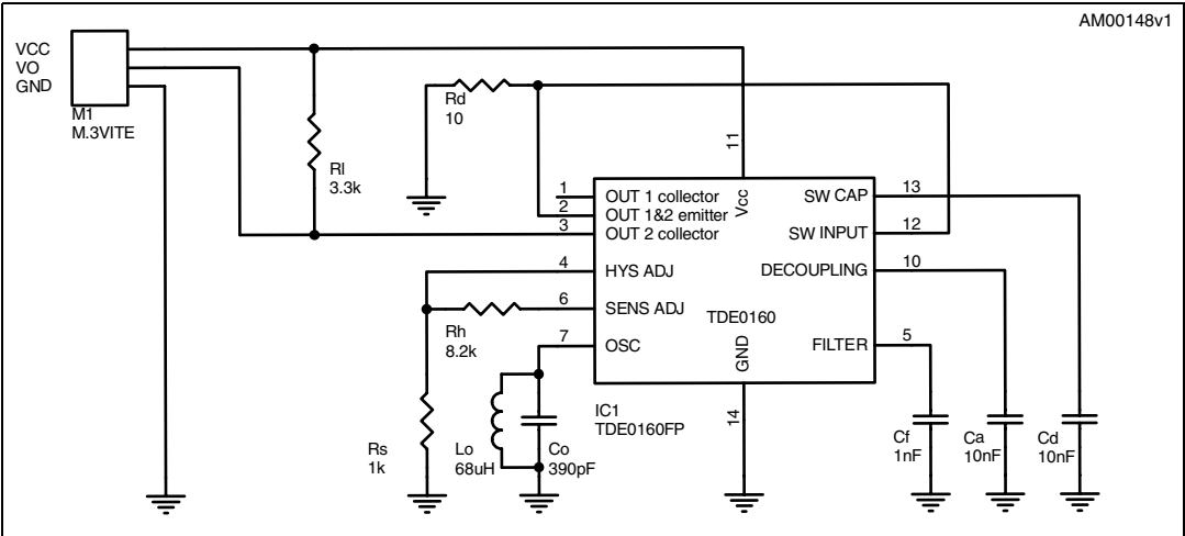
Figure 1. Schematic
