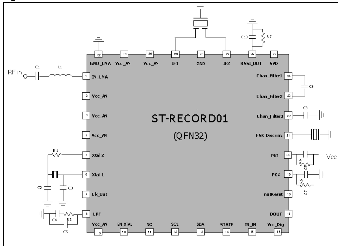
Figure 2. Test circuit
