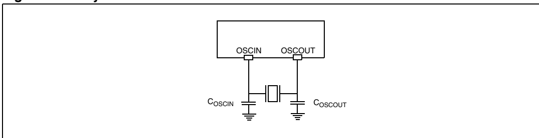
Figure 14. Crystal resonator
