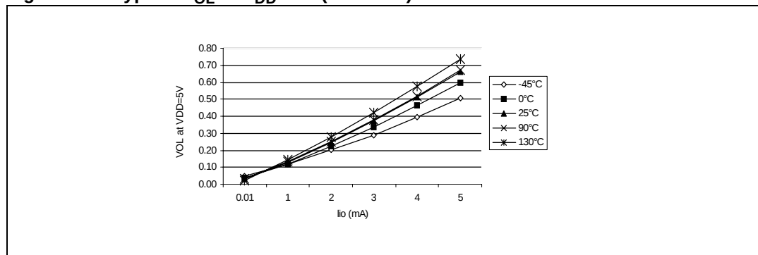
Figure 9. Typical V_{OL} at V_{DD}=5 V (standard)
