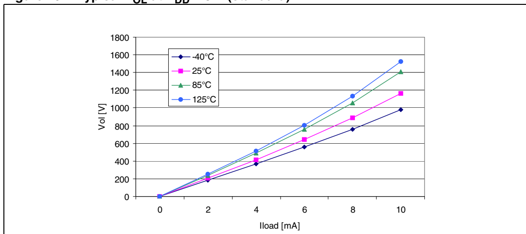
Figure 79. Typical V_{OL} at V_{DD} = 5 V (standard)
