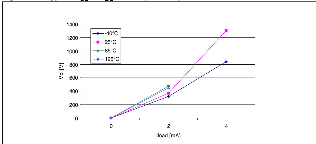
Figure 78. Typical V_{OL} at V_{DD} = 3 V (standard)
