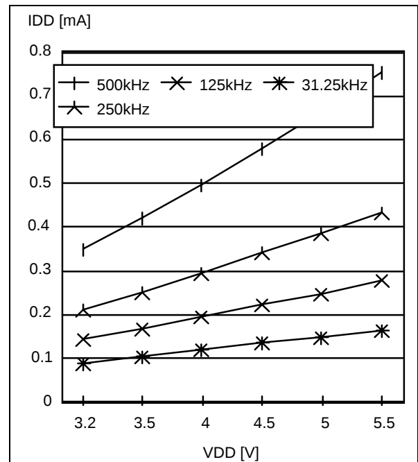
Figure 64. Typical I_{DD} in SLOW vs. f_{CPU}
