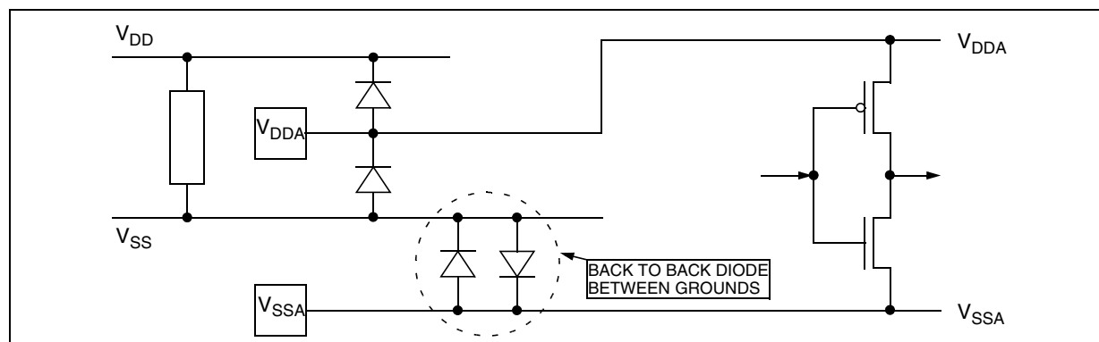
Figure 80. Multisupply Configuration
