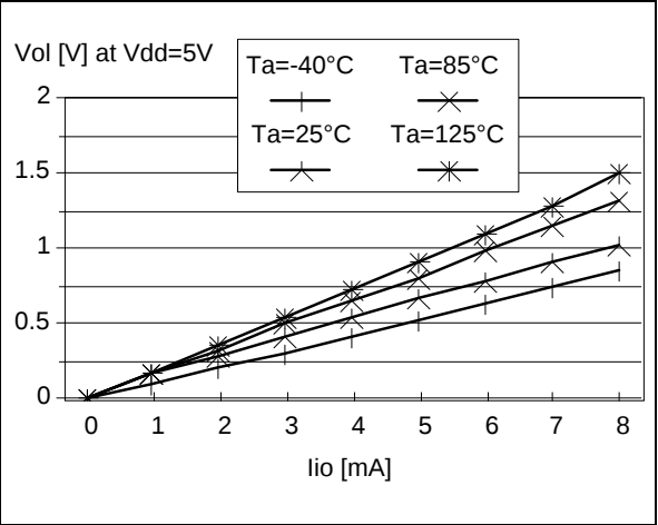
Figure 91. Typical V_{OL} at V_{DD}=5\text{V} (RESET)
