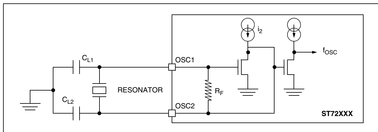
Figure 67. Application with a Crystal Resonator
