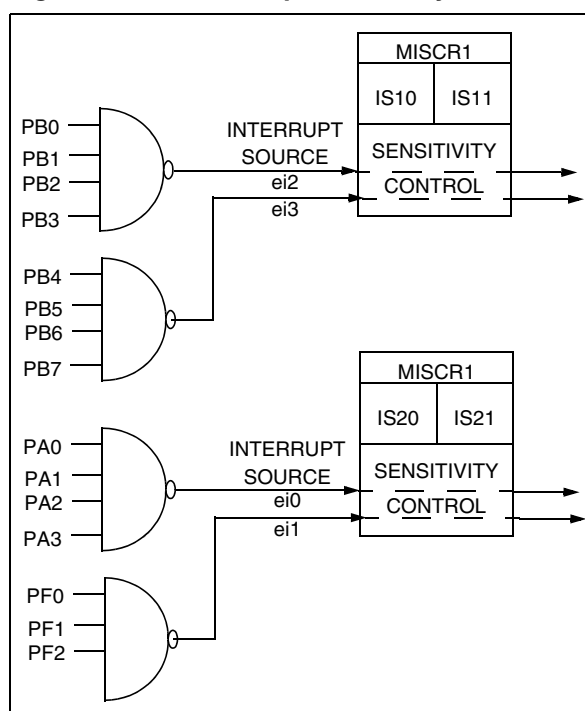
Figure 27. Ext. Interrupt Sensitivity
