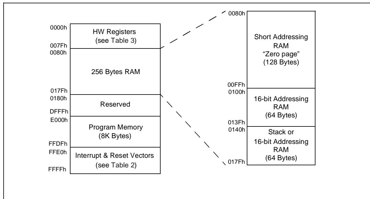
Figure 6. Memory Map
