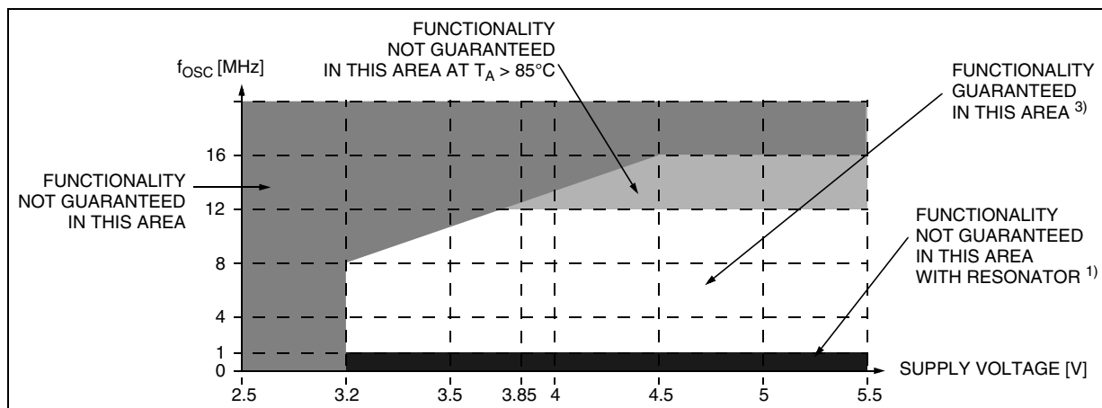
Figure 51. f_{OSC} Maximum Operating Frequency Versus V_{DD} Supply Voltage for Flash devices 2)
