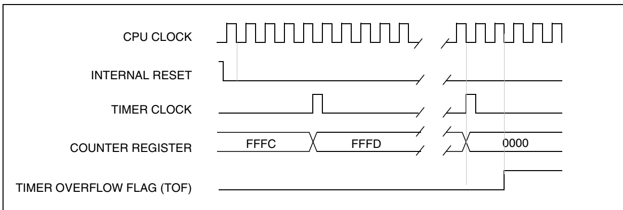
Figure 28. Counter Timing Diagram, internal clock divided by 8
