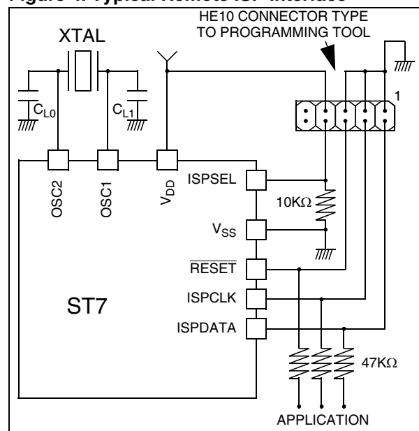
Figure 4. Typical Remote ISP Interface
