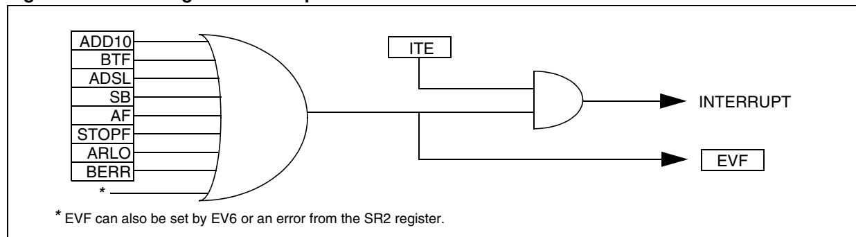
Figure 45. Event Flags and Interrupt Generation
