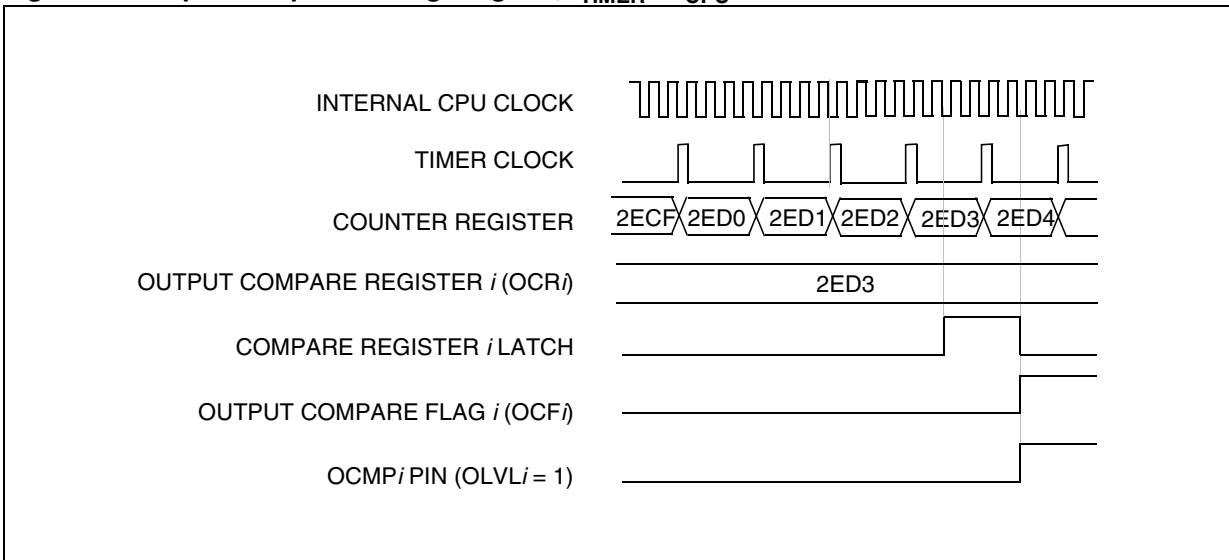
Figure 33. Output Compare Timing Diagram, f_{\text{TIMER}} = f_{\text{CPU}}/4
