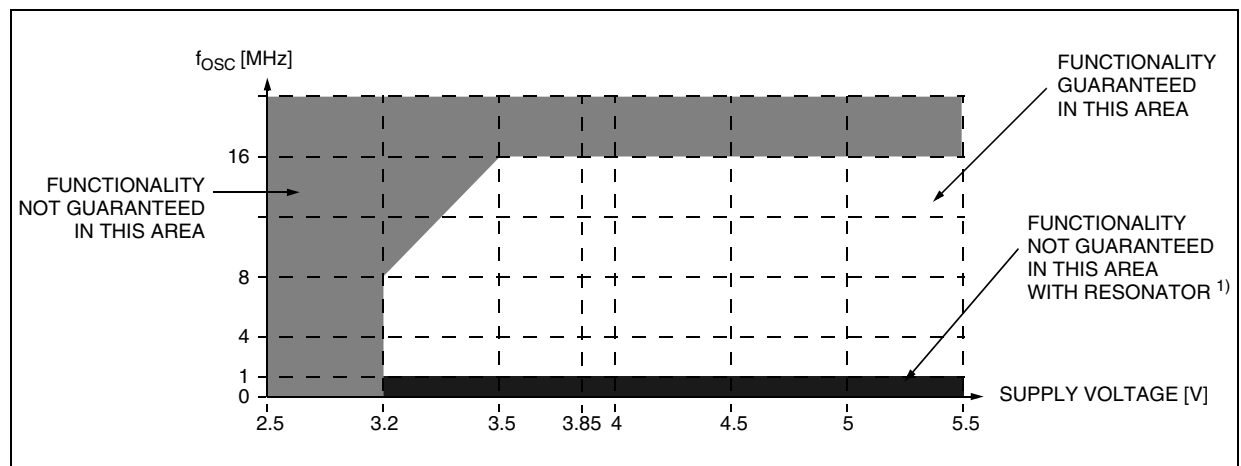
Figure 50. f_{OSC} Maximum Operating Frequency Versus V_{DD} Supply Voltage for ROM Devices 2)
