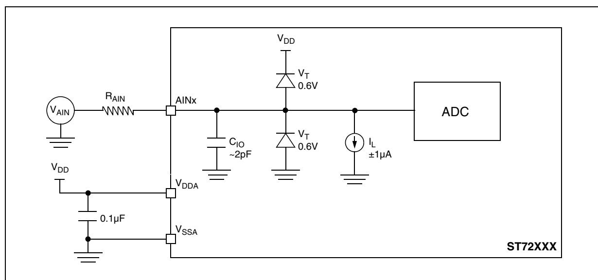
Figure 94. Typical Application with ADC
