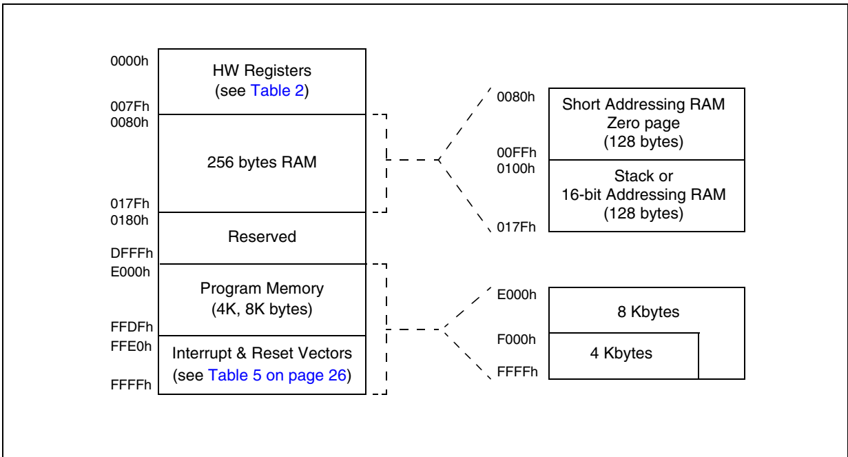
Figure 3. Memory Map
