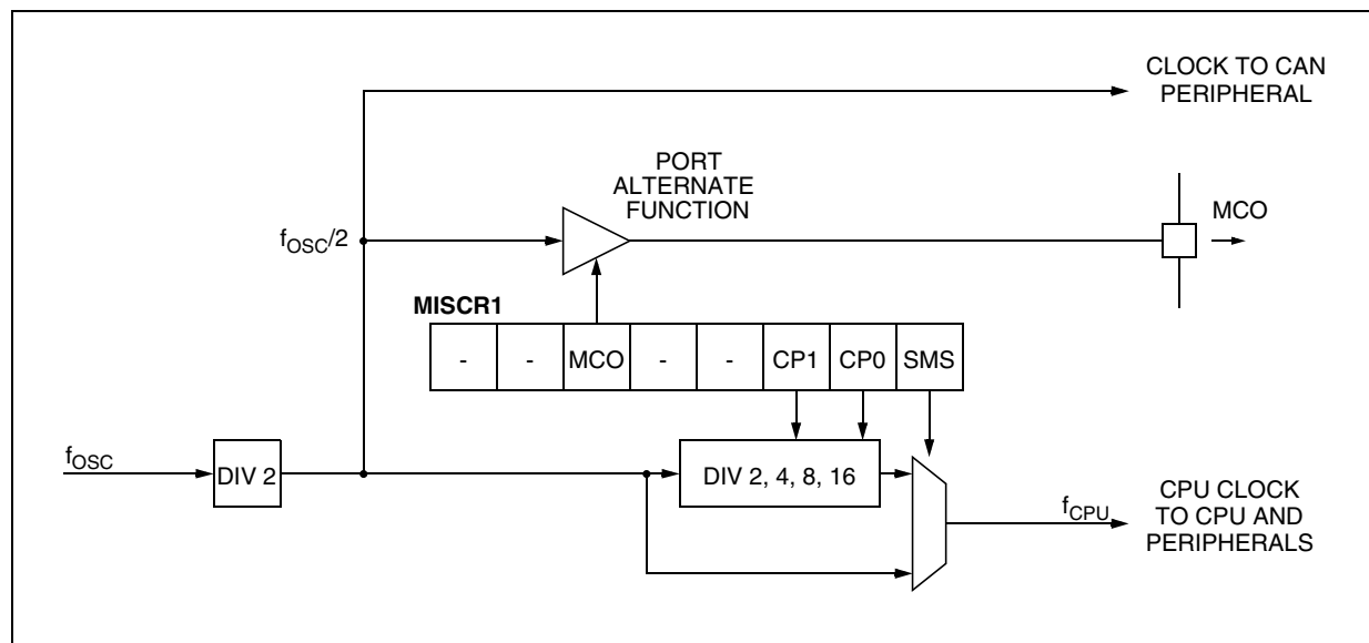
Figure 13. Main Clock Controller (MCC) Block Diagram
