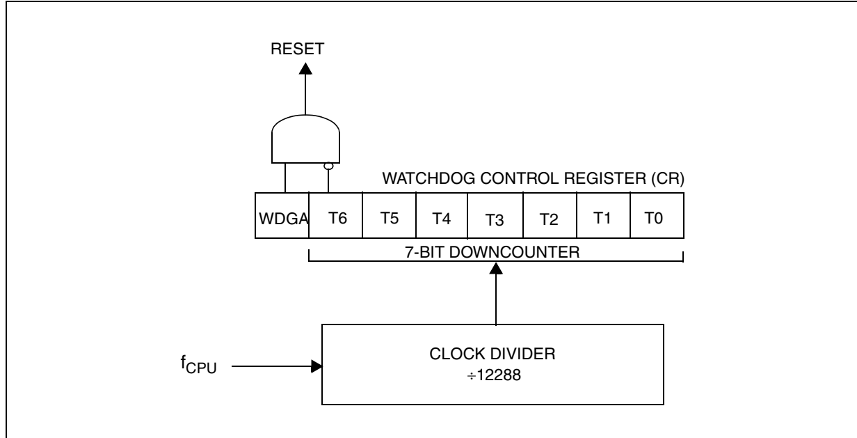
Figure 24. Watchdog Block Diagram
