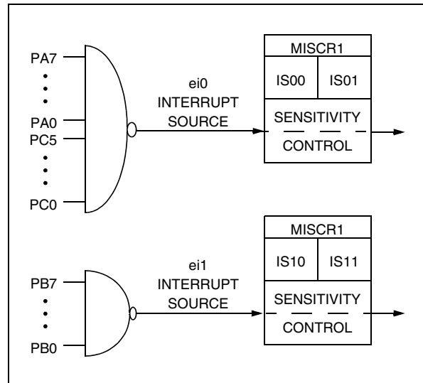
Figure 23. Ext. Interrupt Sensitivity (EXTIT=1)
