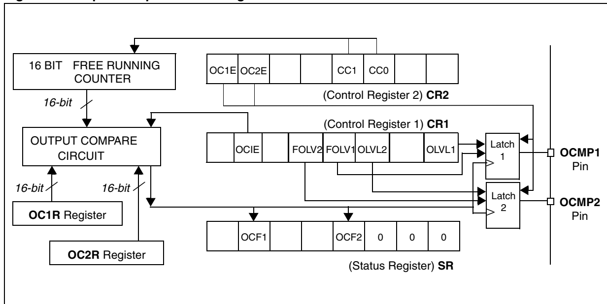
Figure 31. Output Compare Block Diagram
