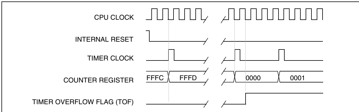
Figure 28. Counter Timing Diagram, internal clock divided by 8
