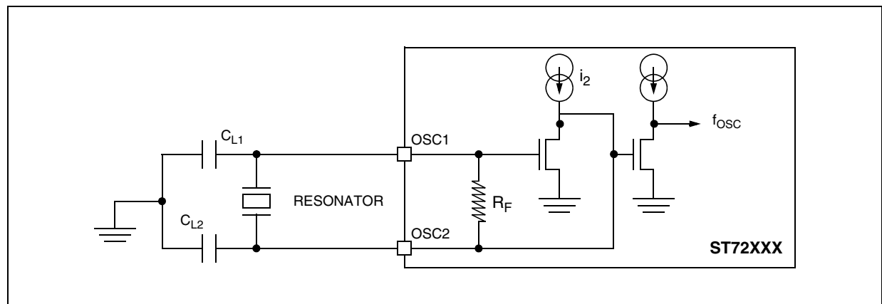
Figure 63. Typical Application with a Crystal Resonator
