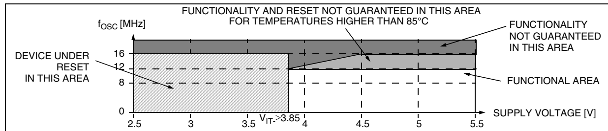
Figure 53. Medium LVD Threshold Versus V_{DD} and f_{OSC} for Flash devices 3)
