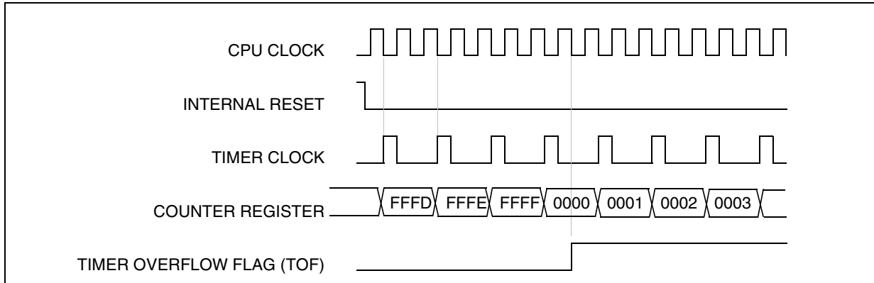
Figure 27. Counter Timing Diagram, internal clock divided by 4
