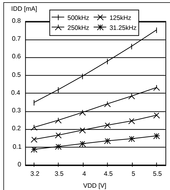
Figure 59. Typical I_{DD} in SLOW vs. f_{CPU}
