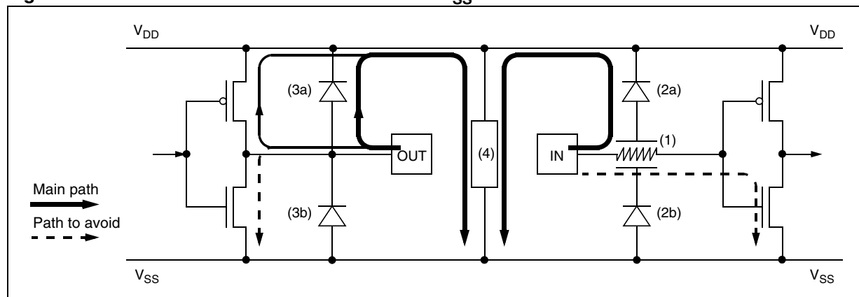
Figure 73. Negative Stress on a Standard Pad vs. V_{DD}
