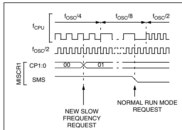
Figure 16. SLOW Mode Clock Transitions
