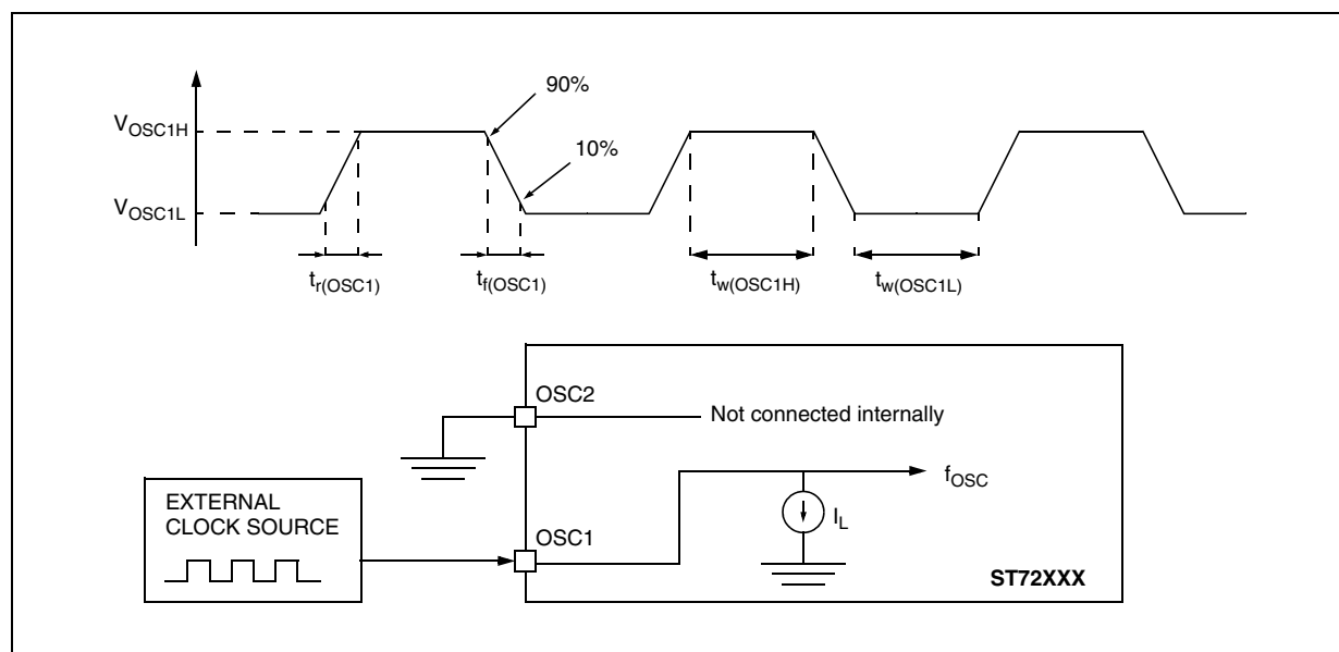
Figure 62. Typical Application with an External Clock Source
