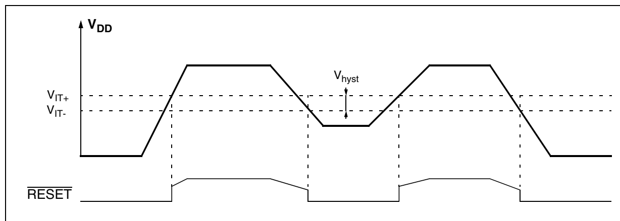
Figure 8. Low Voltage Detector vs Reset
