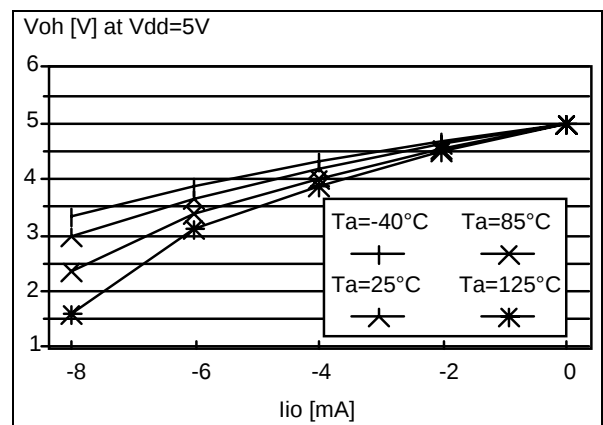
Figure 81. Typical V_{OH} at V_{DD}=5V
