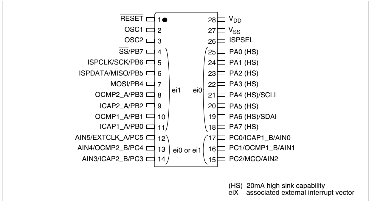
Figure 2. 28-Pin SO Package Pinout
