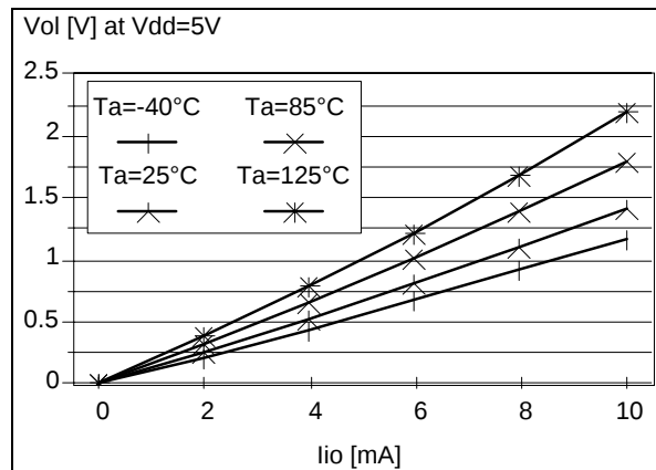
Figure 80. Typical V_{OL} at V_{DD}=5V (high-sink)
