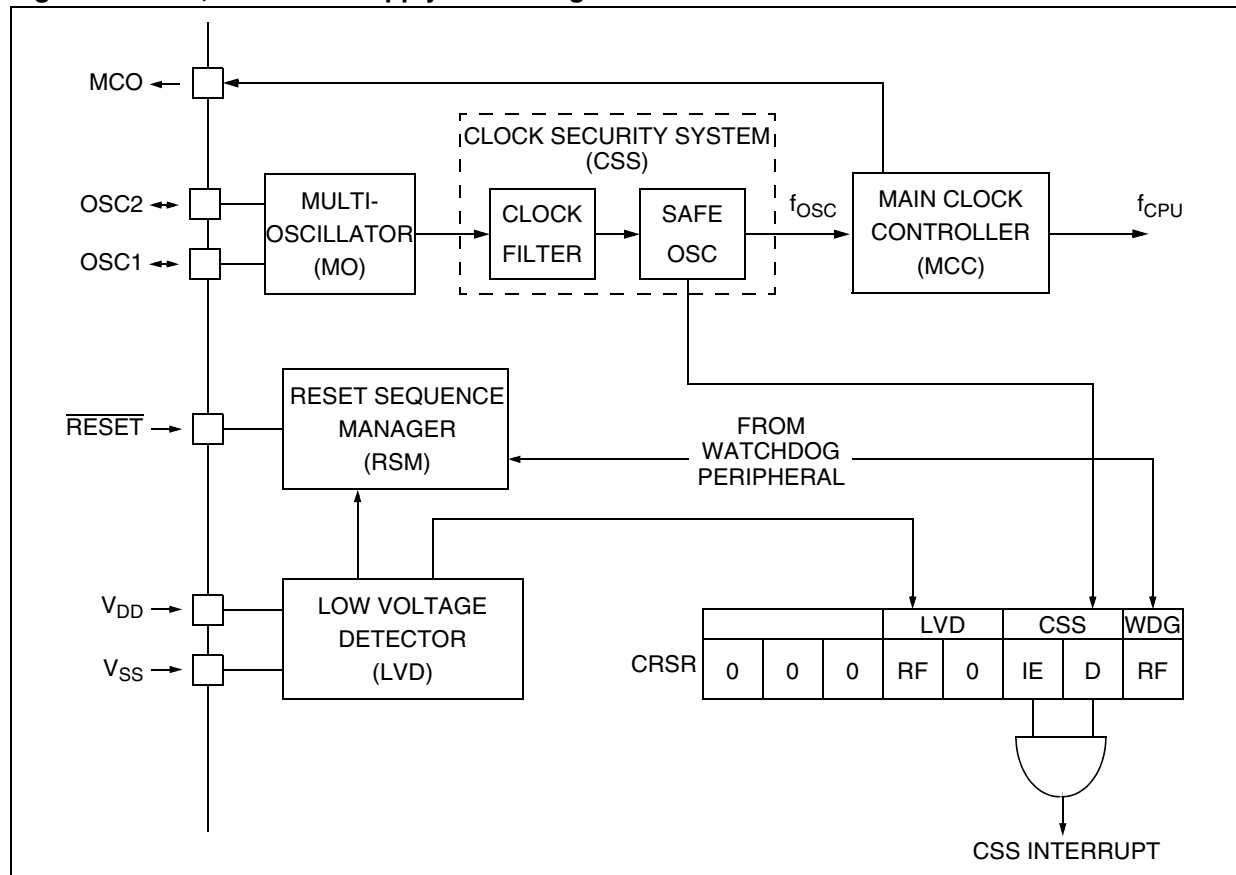
Figure 7. Clock, Reset and Supply Block Diagram
