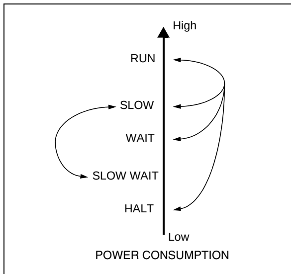
Figure 15. Power Saving Mode Transitions
