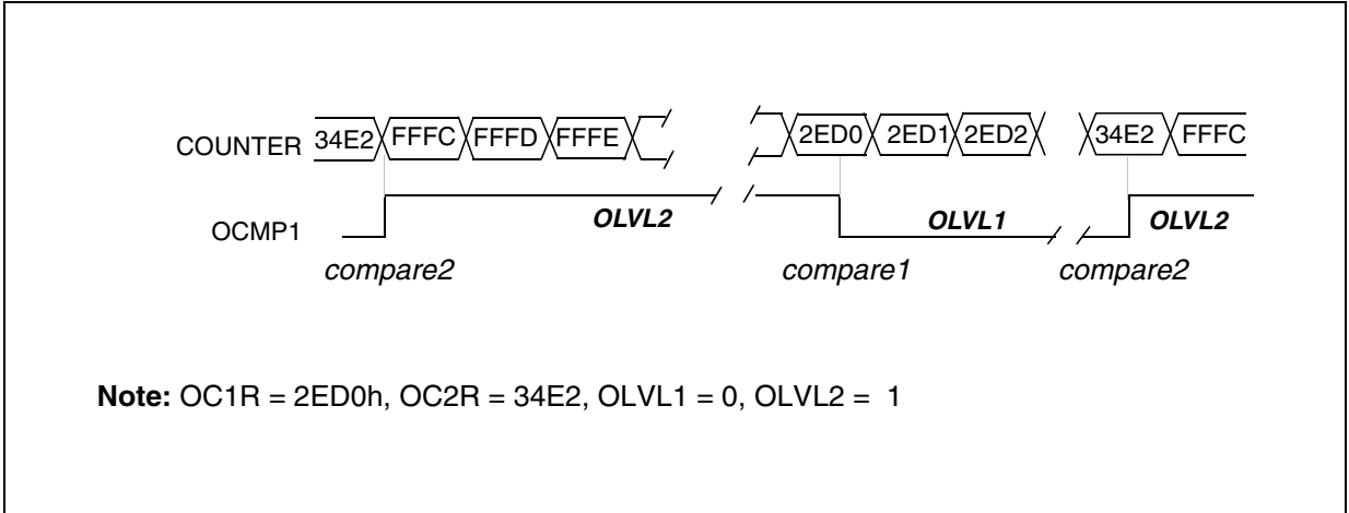
Figure 35. Pulse Width Modulation Mode Timing Example
