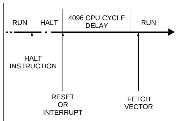
Figure 18. HALT Mode Timing Overview
