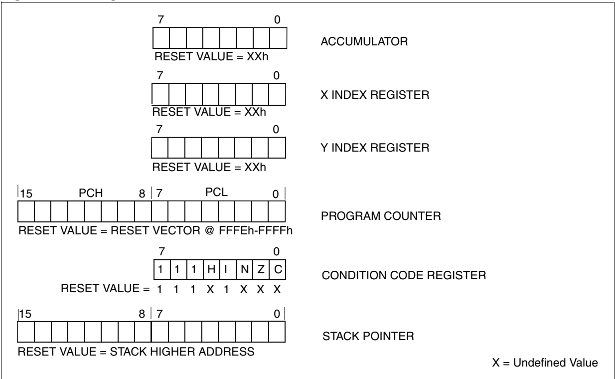
Figure 5. CPU Registers
