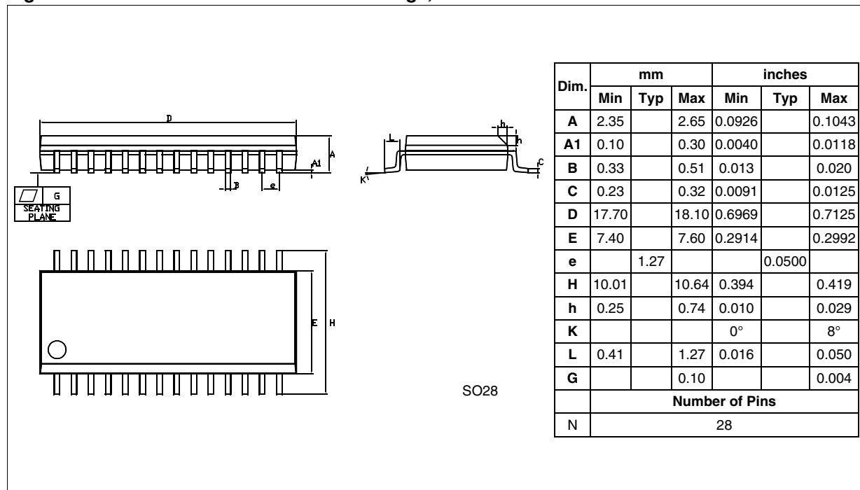
Figure 96. 28-Pin Plastic Small Outline Package, 300-mil Width
