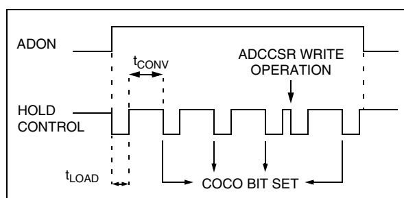
Figure 47. ADC Conversion Timings
