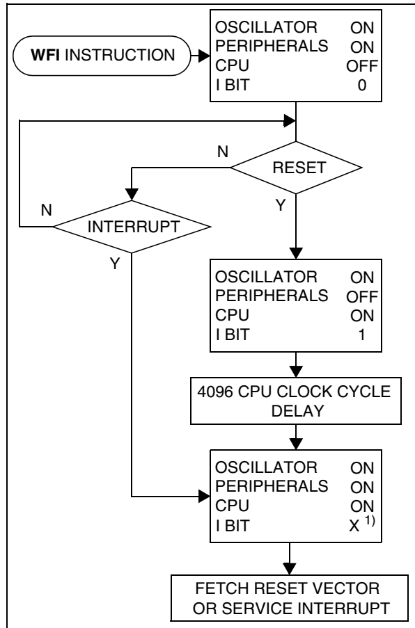
Figure 17. WAIT Mode Flowchart
