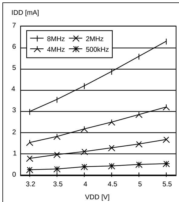
Figure 58. Typical I_{DD} in RUN vs. f_{CPU}
