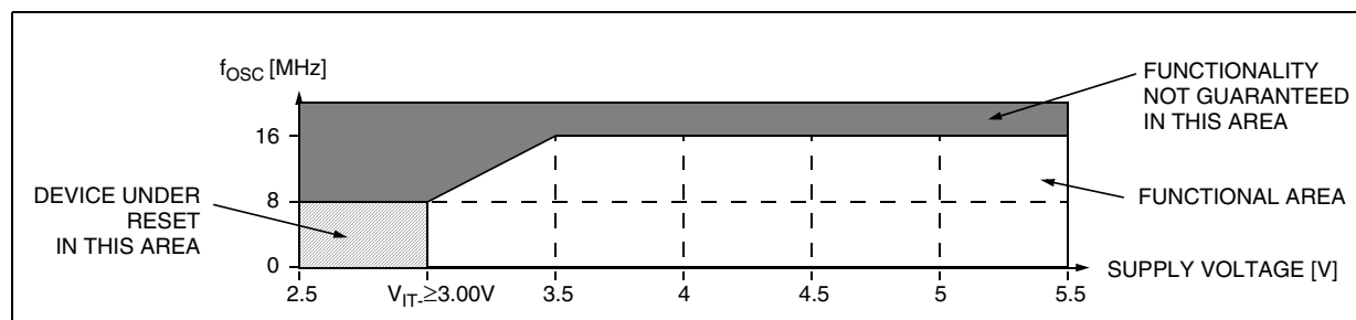
Figure 57. Low LVD Threshold Versus V_{DD} and f_{OSC} for ROM devices 2)3)
