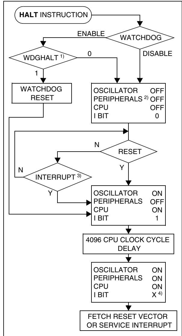
Figure 19. HALT Mode Flow-chart
