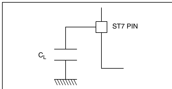
Figure 48. Pin Loading Conditions
