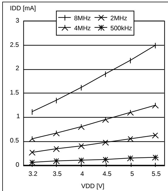
Figure 60. Typical I_{DD} in WAIT vs. f_{CPU}
