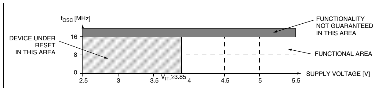
Figure 56. Medium LVD Threshold Versus V_{DD} and f_{OSC} for ROM devices 2)
