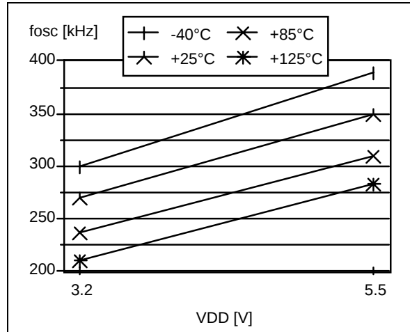
Figure 68. Typical Safe Oscillator Frequencies
