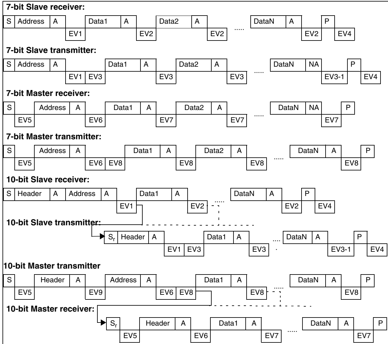
Figure 44. Transfer Sequencing
