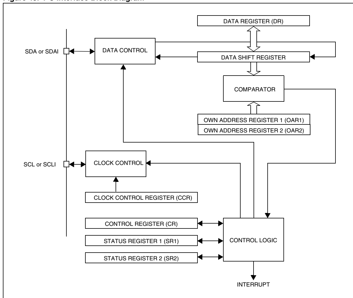
Figure 43. I 2 C Interface Block Diagram
