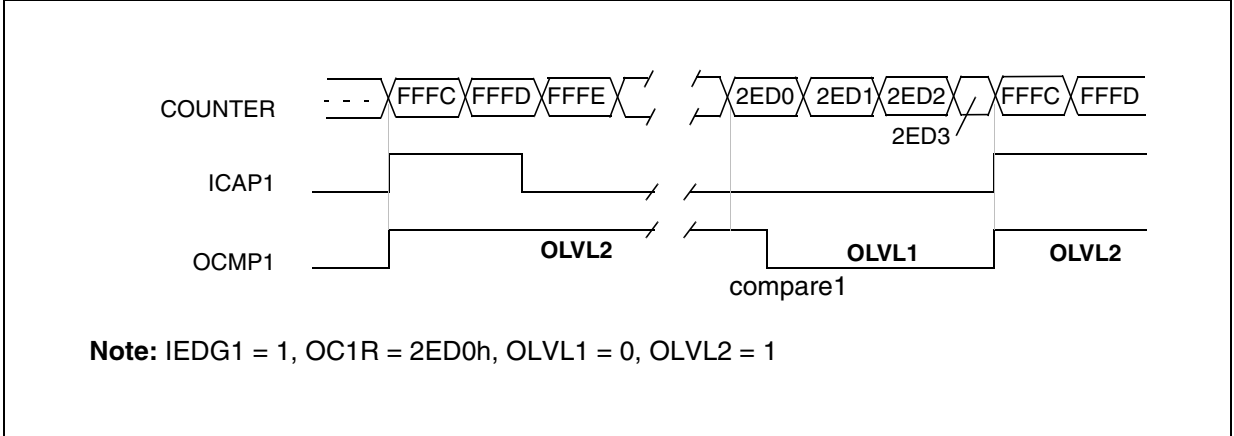
Figure 34. One Pulse Mode Timing Example
