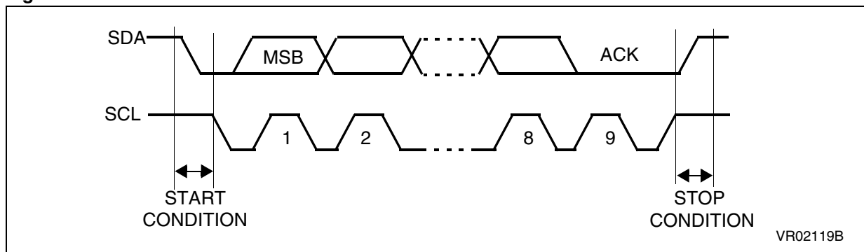
Figure 42. I 2 C BUS Protocol
