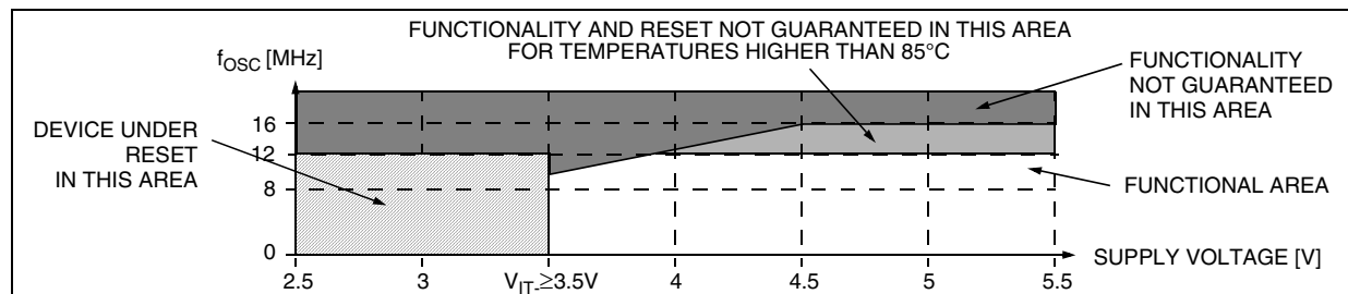
Figure 54. Low LVD Threshold Versus V_{DD} and f_{OSC} for Flash devices 2)4)
