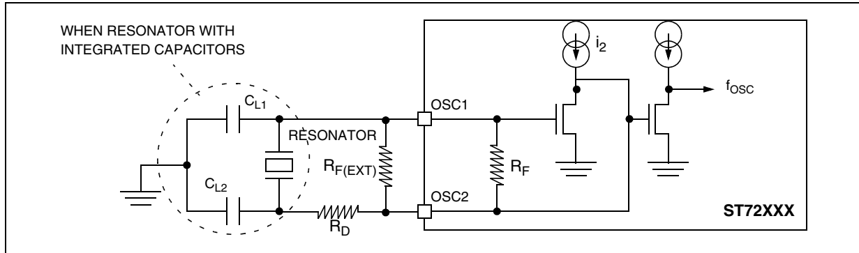
Figure 64. Typical Application with Ceramic Resonator
