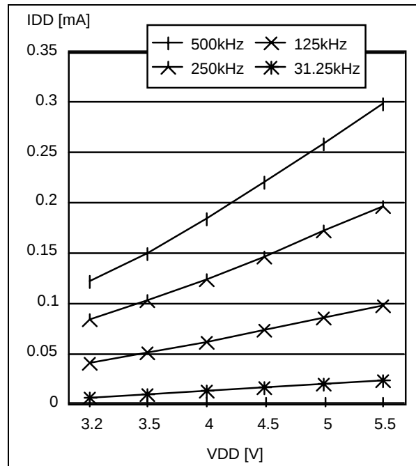
Figure 61. Typical I_{DD} in SLOW-WAIT vs. f_{CPU}
