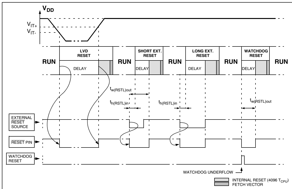
Figure 11. RESET Sequences
