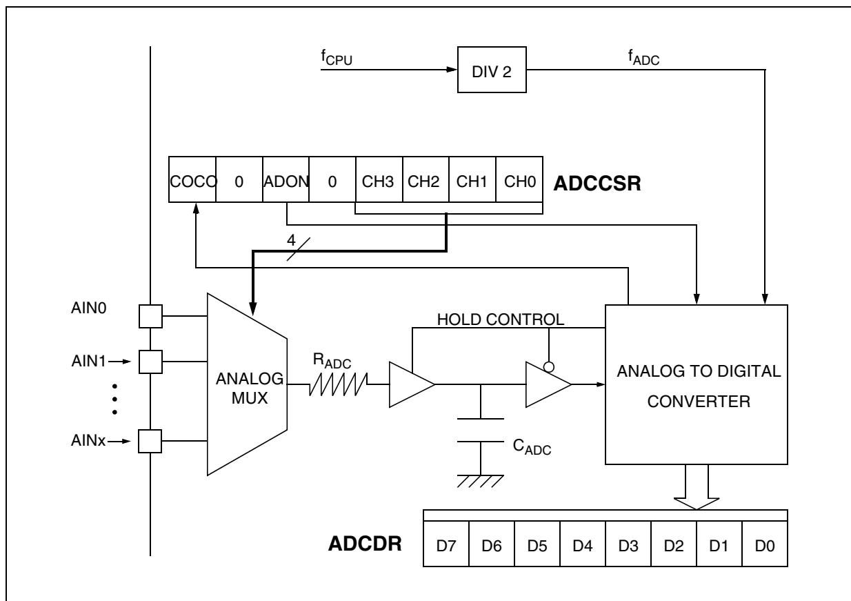
Figure 46. ADC Block Diagram
