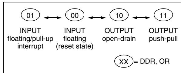
Figure 21. Interrupt I/O Port State Transitions
