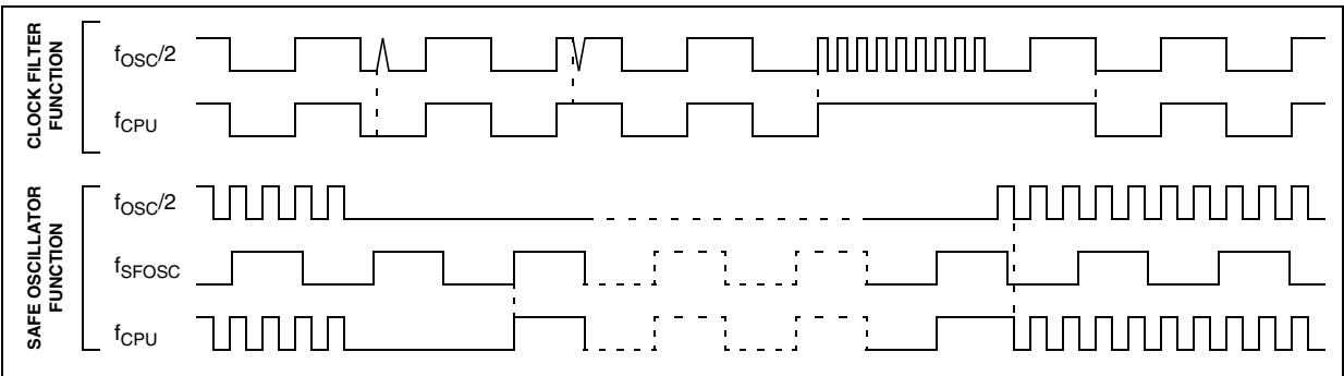
Figure 12. Clock Filter Function and Safe Oscillator Function
