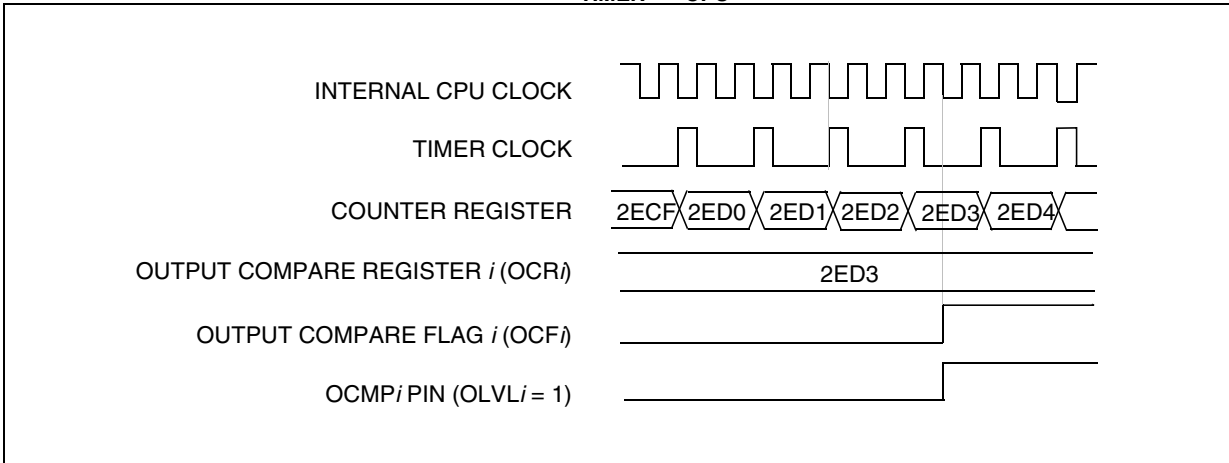
Figure 32. Output Compare Timing Diagram, f_{\text{TIMER}} = f_{\text{CPU}}/2
