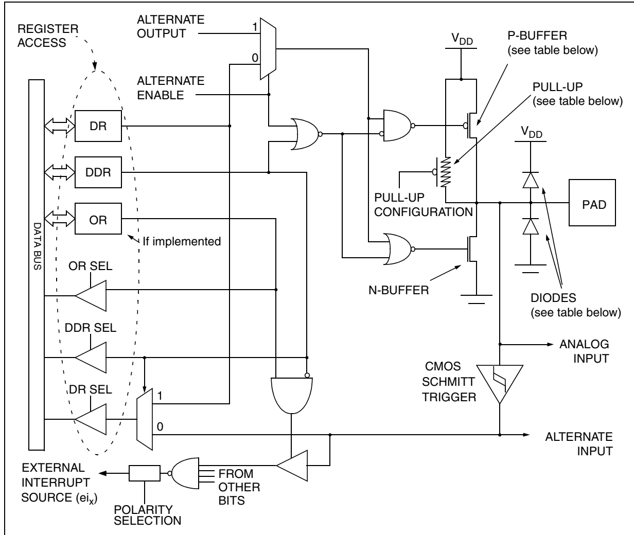
Figure 20. I/O Port General Block Diagram
