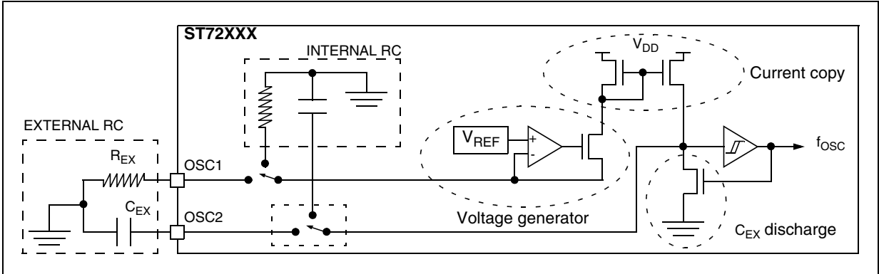
Figure 66. Typical Internal RC Oscillator
