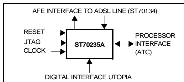
Figure 9 : ST70235A Interfaces
