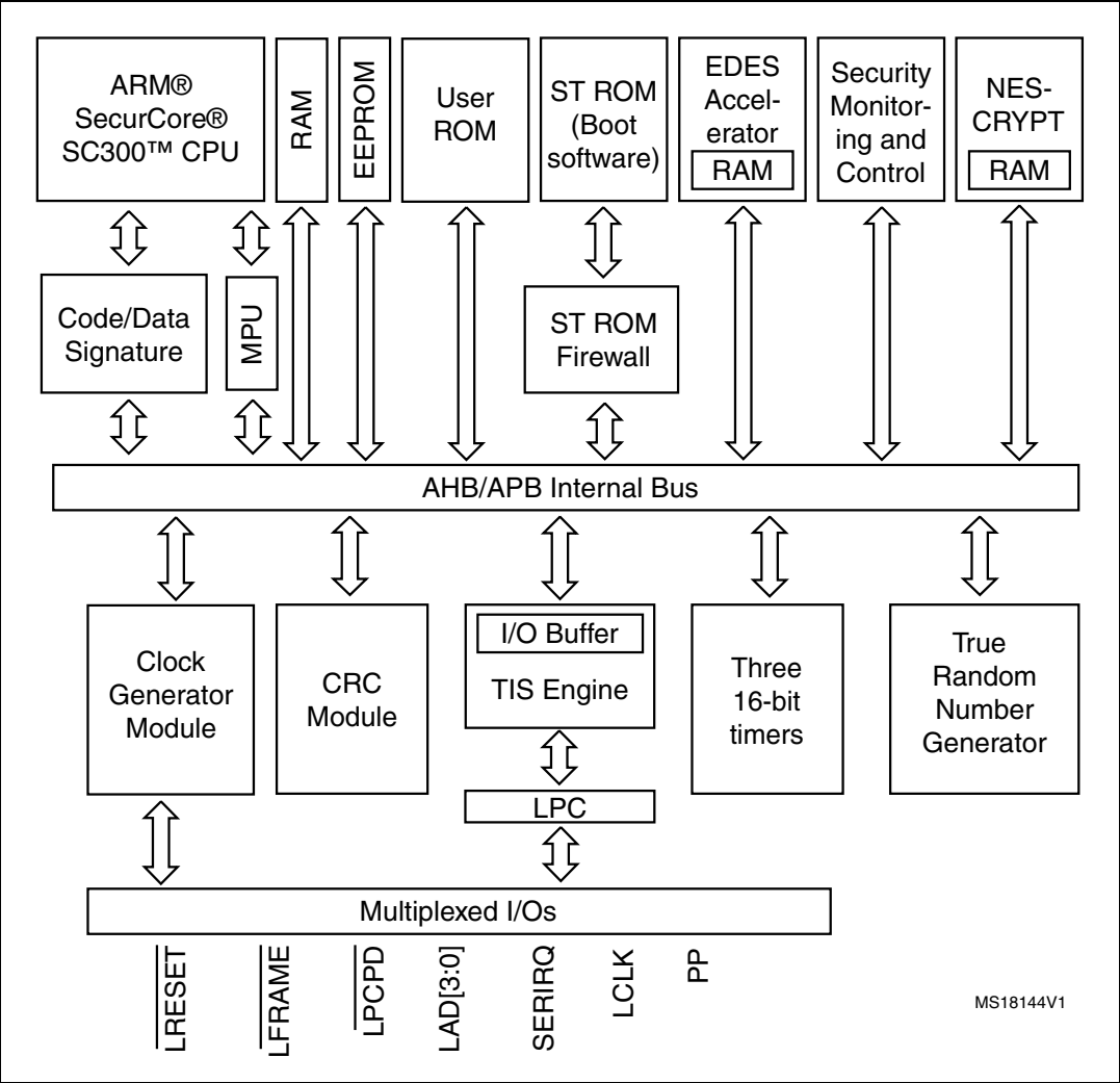
Figure 1. ST33TPM12LPC block diagram
