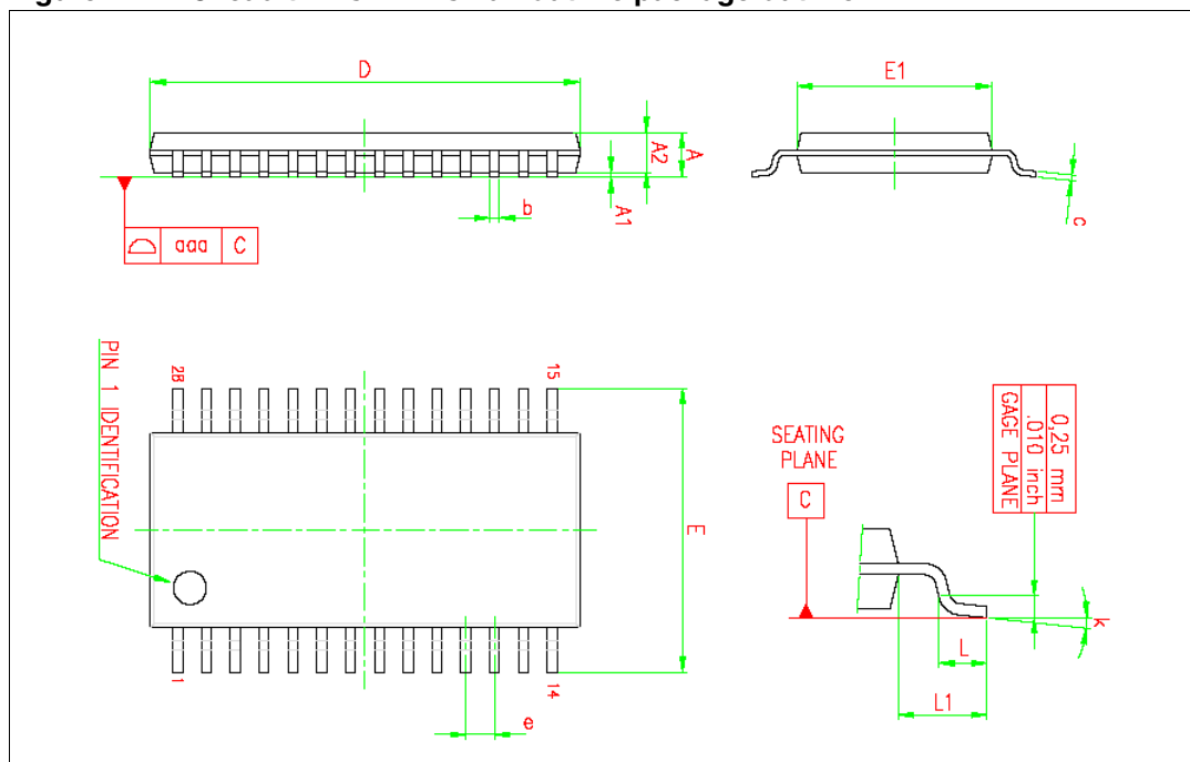
Figure 4. 28-lead thin shrink small outline package outline
