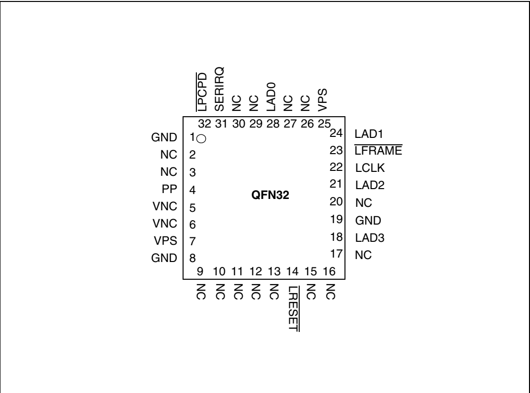
Figure 3. QFN32 pinout
