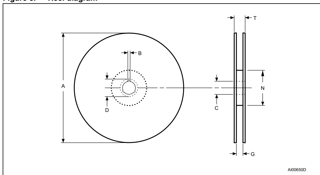
Figure 6. Reel diagram
