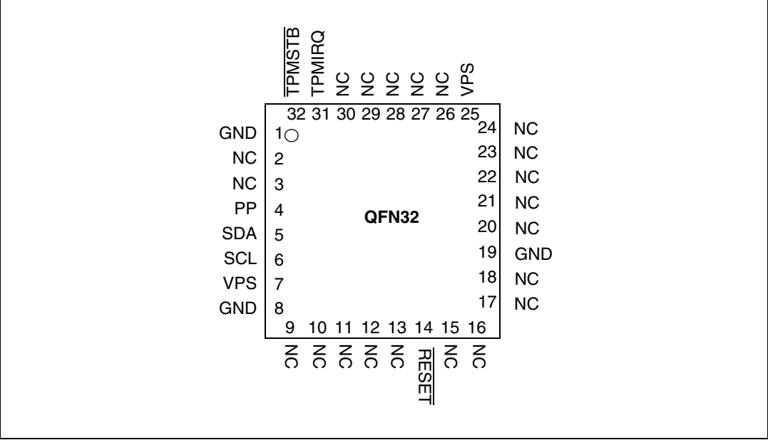
Figure 3. VQFN32 pinout
