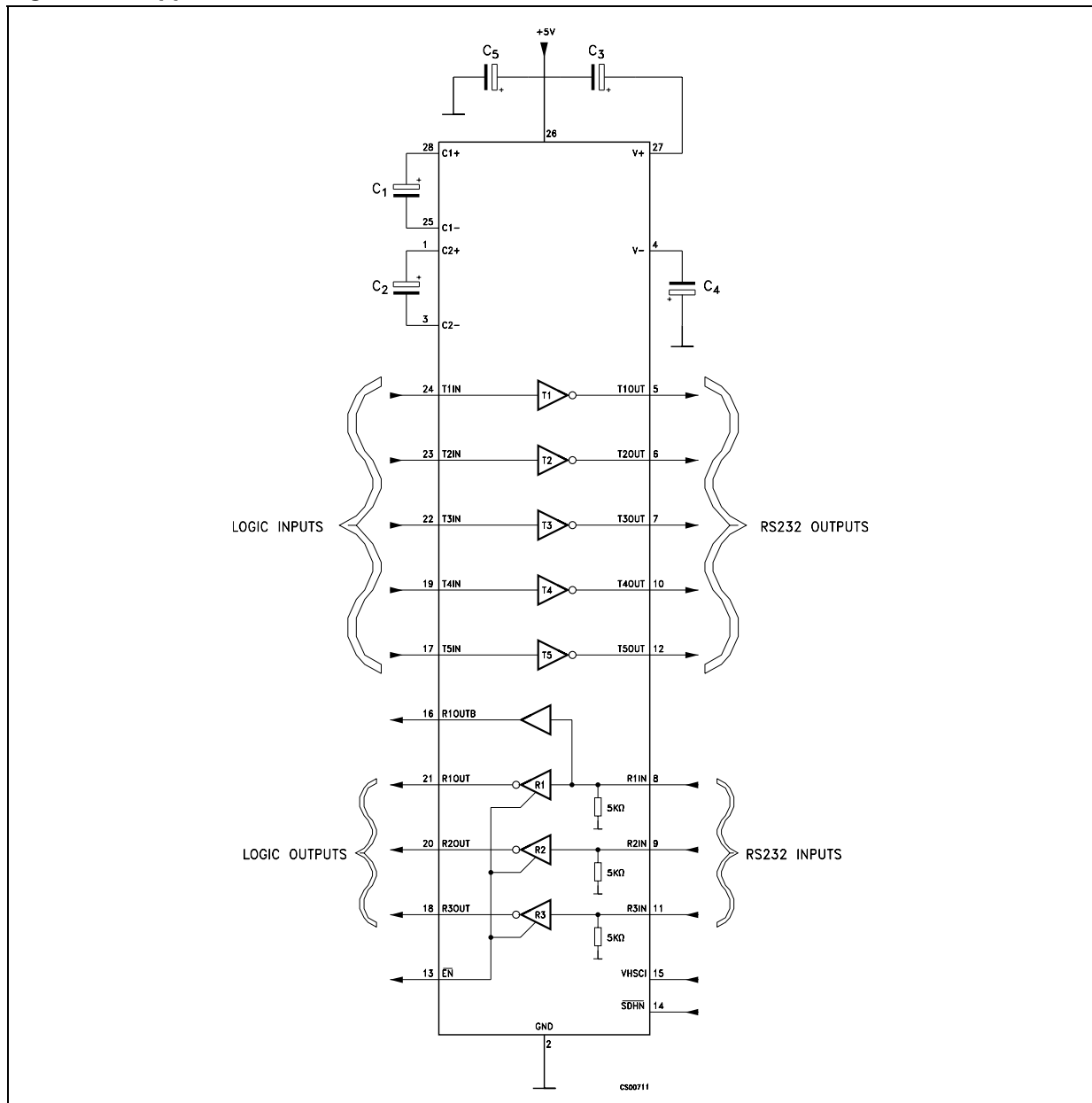
Figure 3. Application circuits
