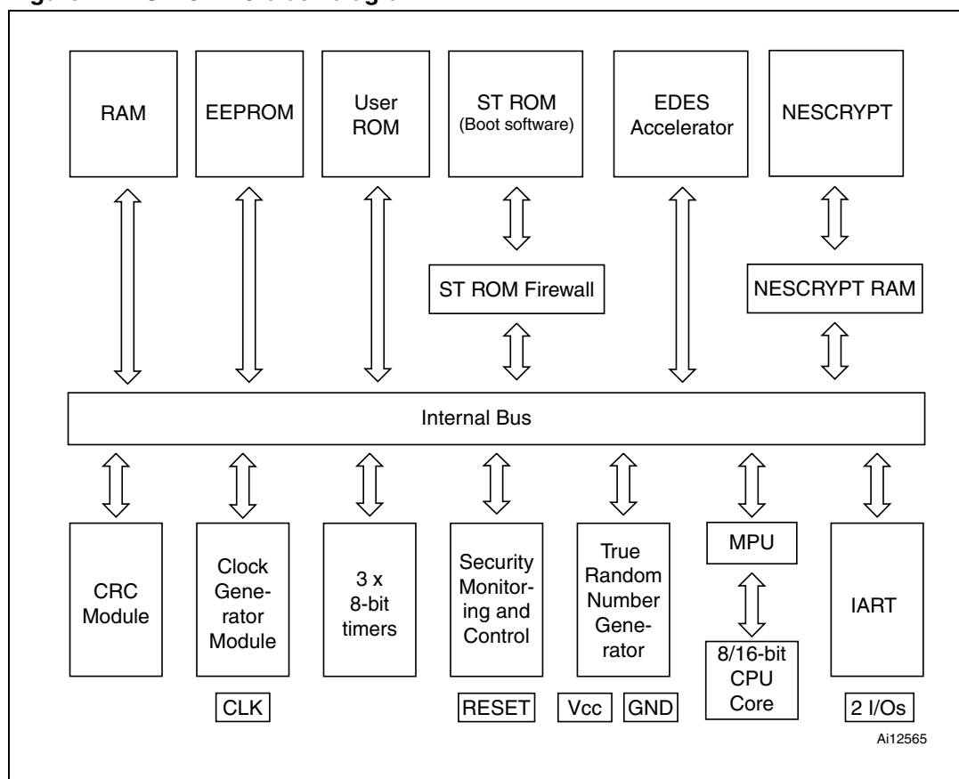
Figure 1. ST23ZL48 block diagram
