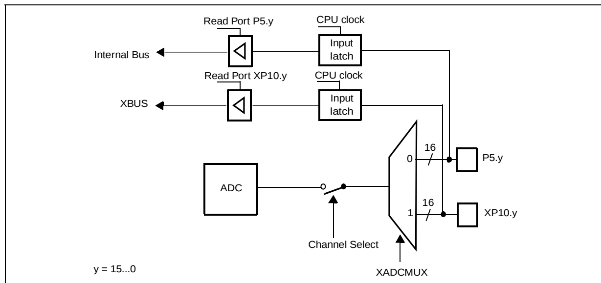
Figure 52 : Block Diagram
