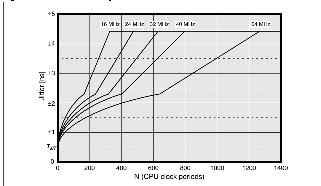
Figure 53. ST10F276E PLL jitter
