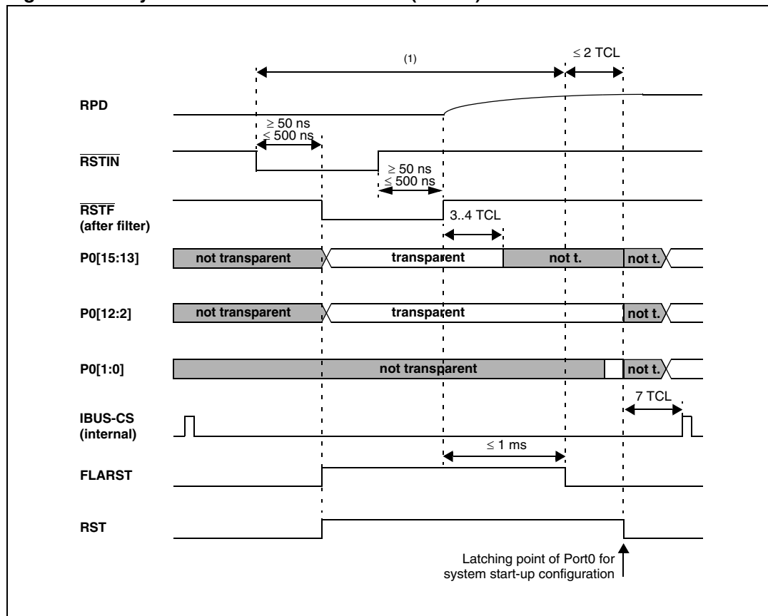
Figure 26. Asynchronous hardware RESET ( \overline{EA} = 1 )
