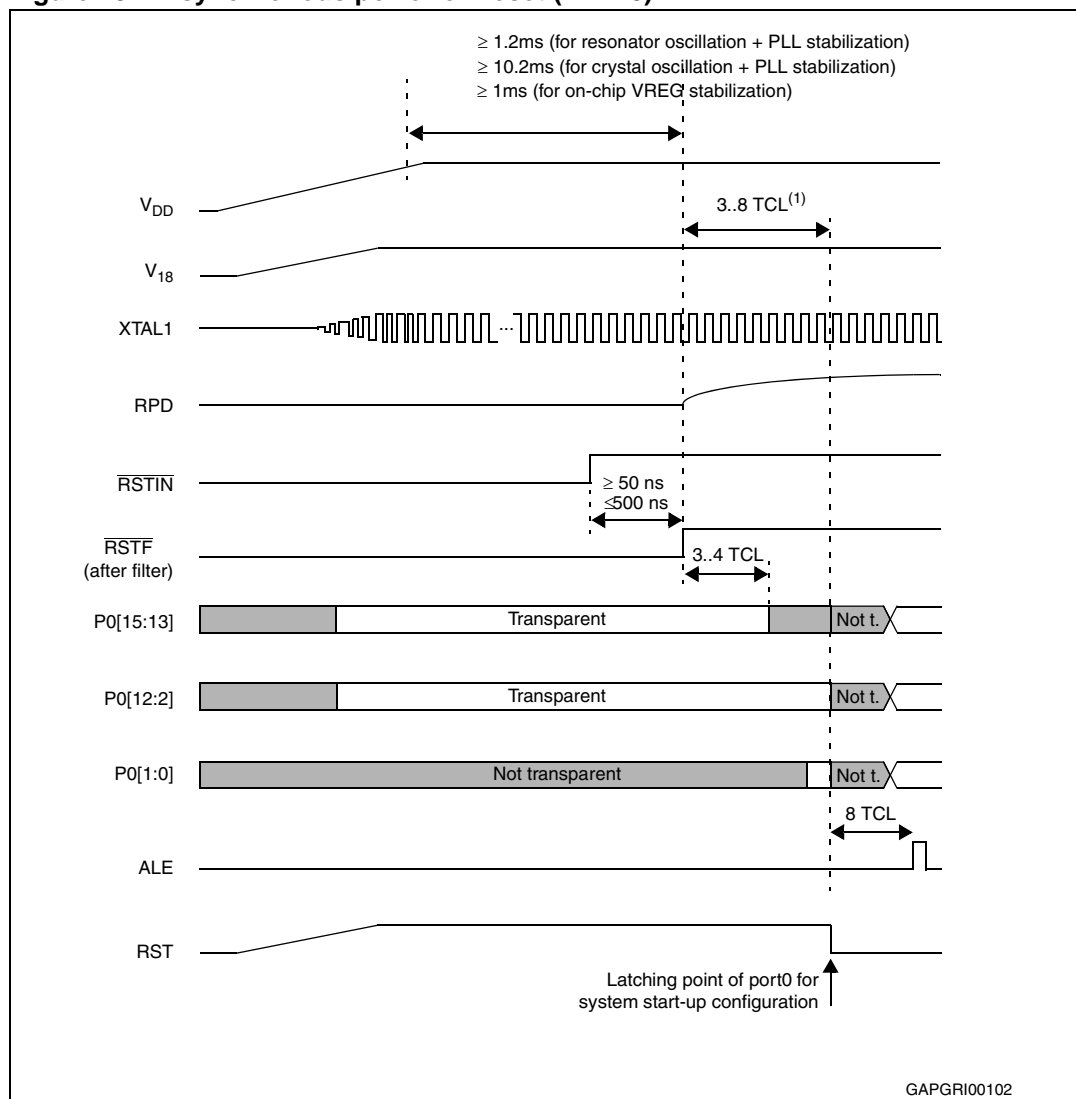
Figure 18. Asynchronous power-on reset ( \overline{EA} = 0 )
