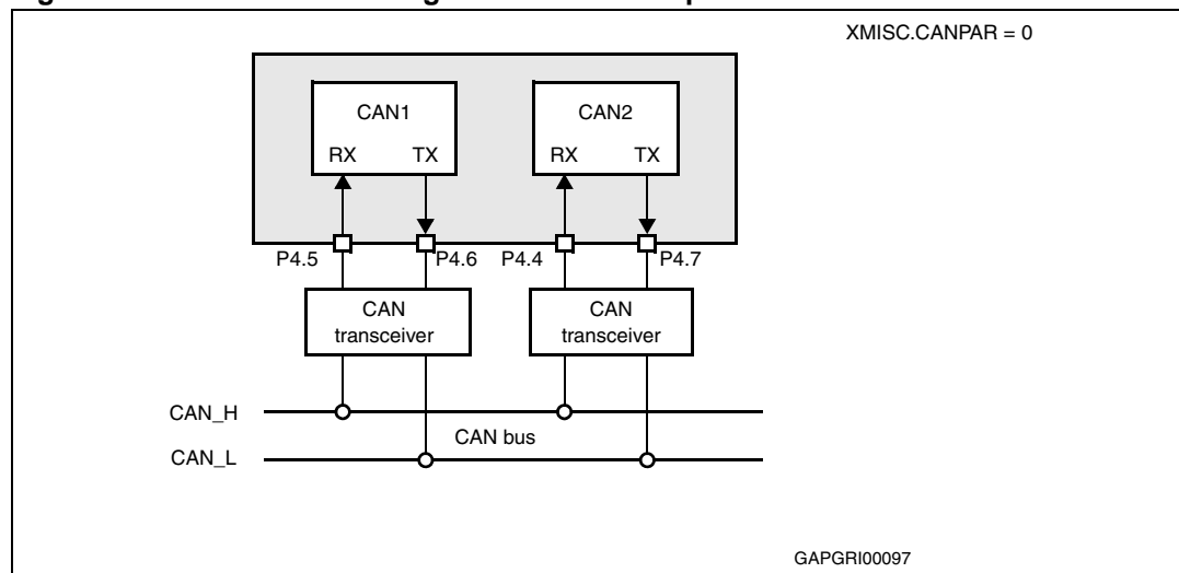
Figure 13. Connection to single CAN bus via separate CAN transceivers
