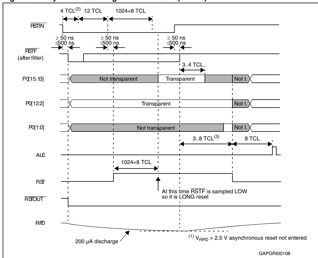
Figure 24. Synchronous long hardware reset ( \overline{\text{EA}} = 0 )
