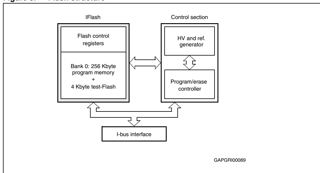
Figure 5. Flash structure
