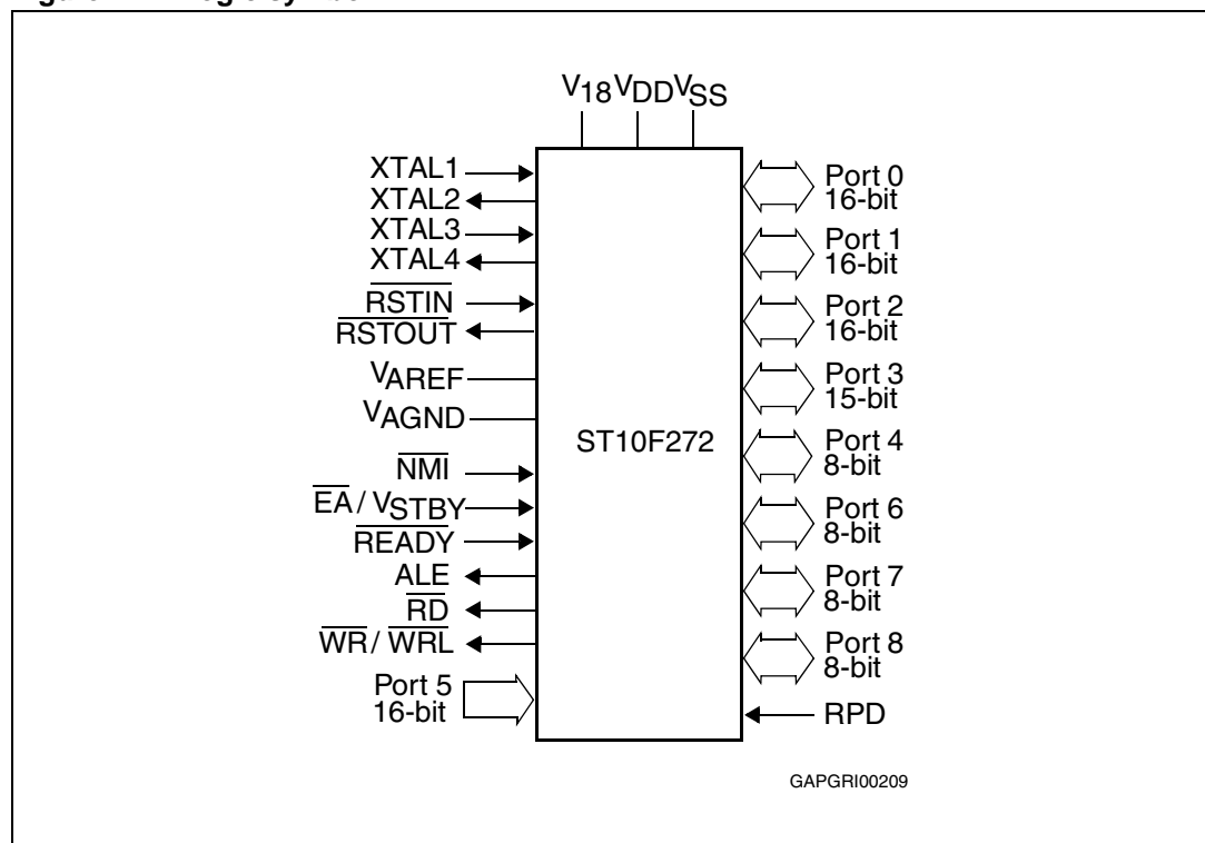
Figure 1. Logic symbol
