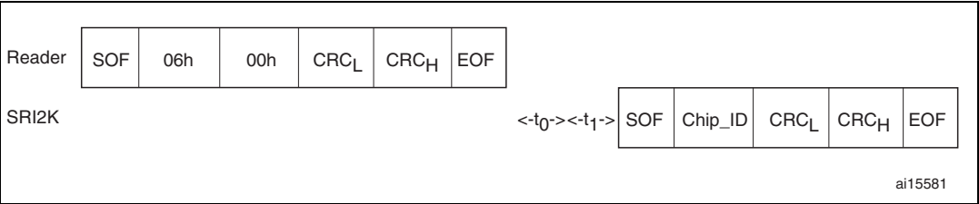
Figure 52. Initiate frame exchange between reader and SRI2K
