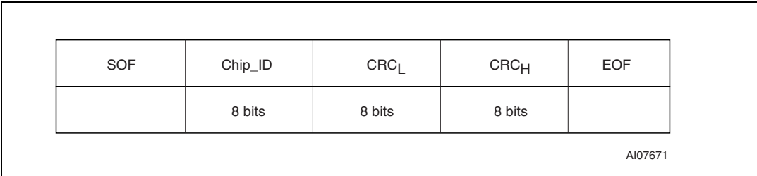
Figure 27. Pcall16 response format
