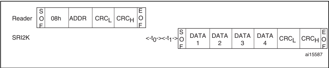
Figure 58. Read_block frame exchange between reader and SRI2K
