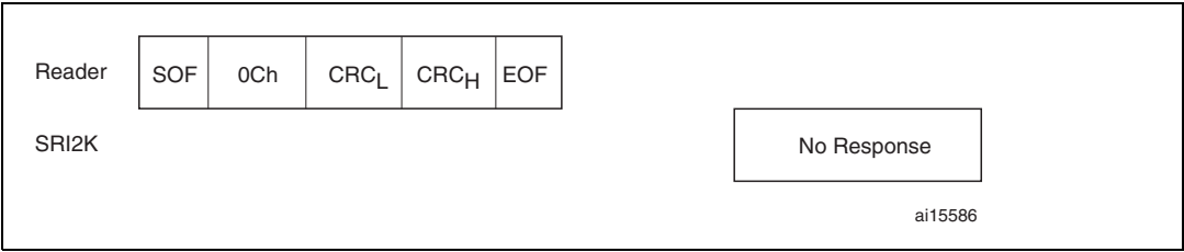
Figure 57. Reset_to_inventory frame exchange between reader and SRI2K
