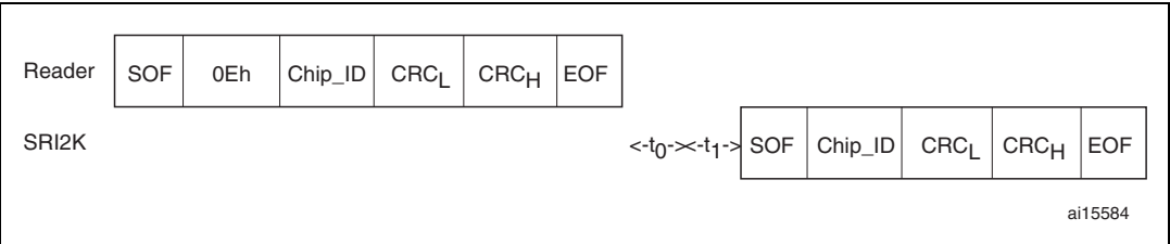
Figure 55. Select frame exchange between reader and SRI2K
