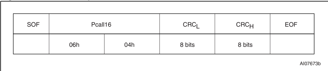
Figure 26. Pcall16 request format
