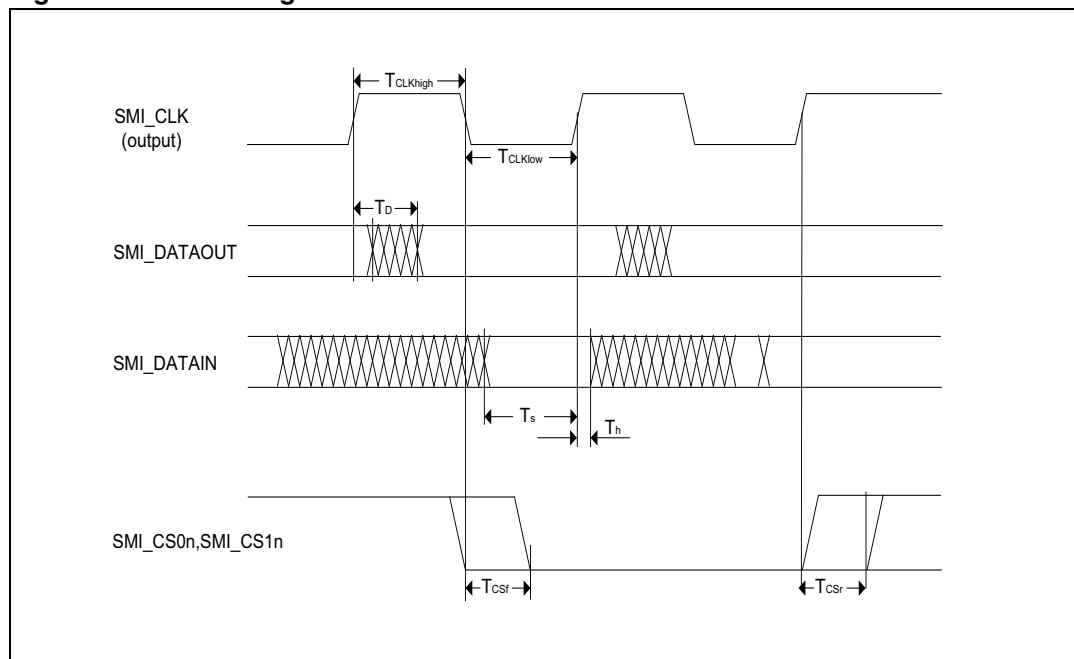
Figure 41. SMI timing waveform
