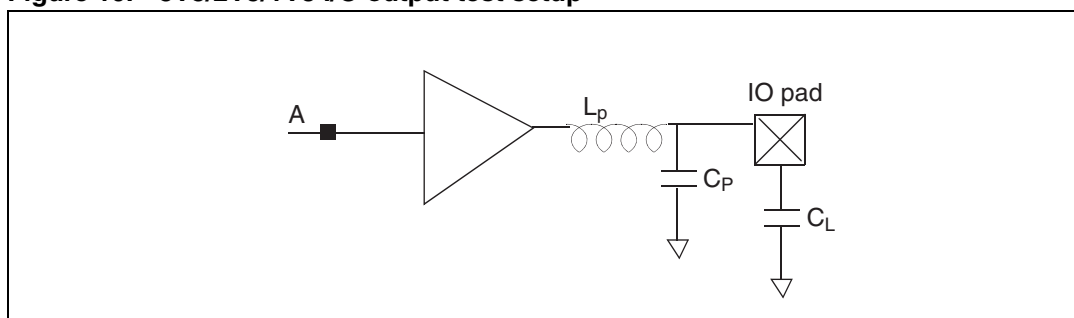
Figure 10. 3V3/2V5/1V8 I/O output test setup
