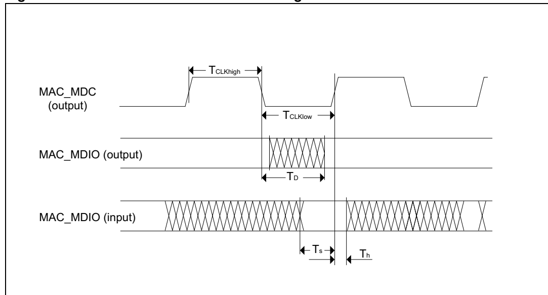
Figure 34. MCIF - SD/SDIO/MMC mode timing waveform
