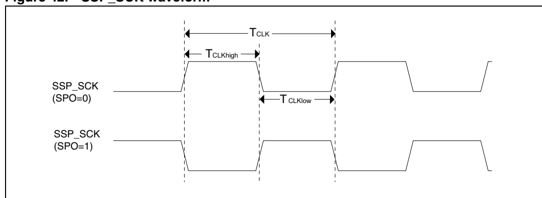
Figure 42. SSP_SCK waveform
