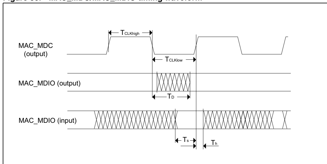
Figure 30. MAC_MDC/MAC_MDIO timing waveform
