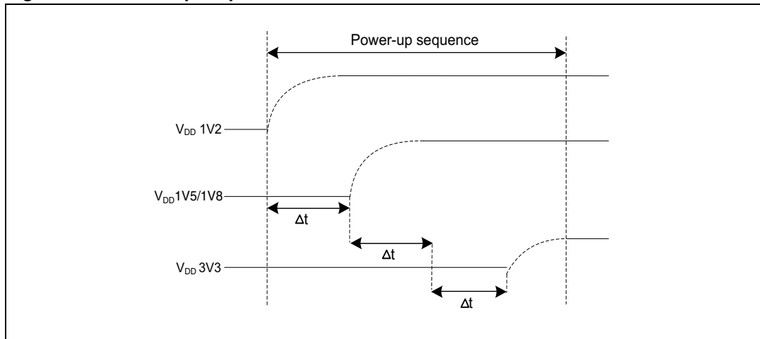
Figure 13. Power-up sequence
