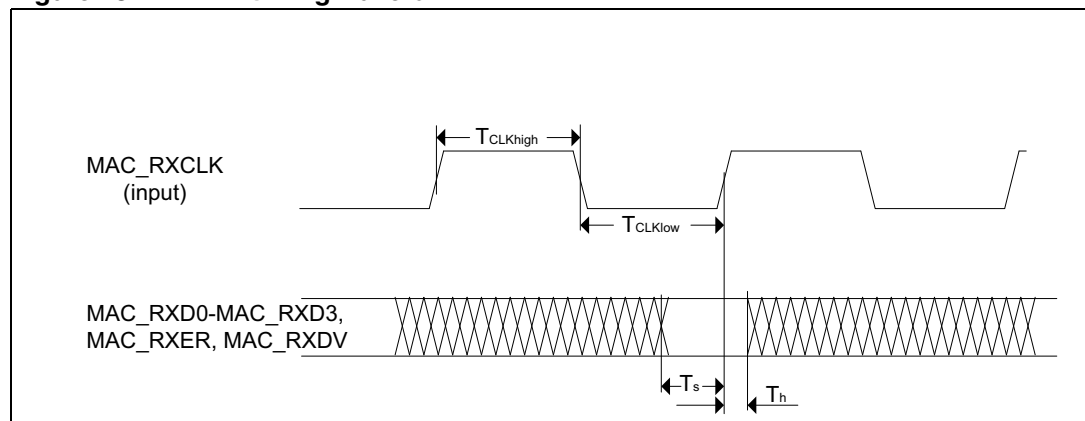
Figure 28. MII RX timing waveform
