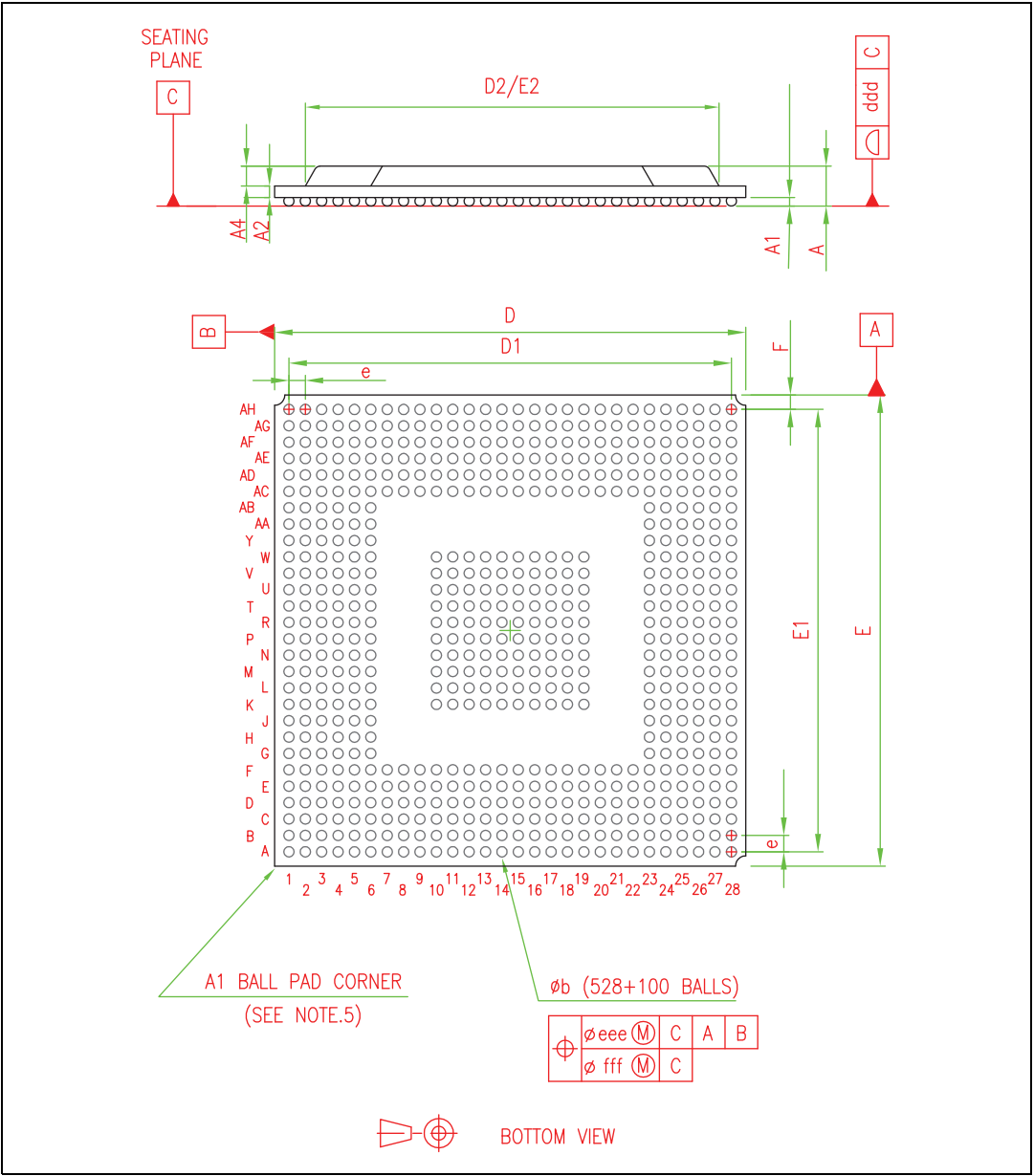
Figure 50. PGBA package - bottom view
