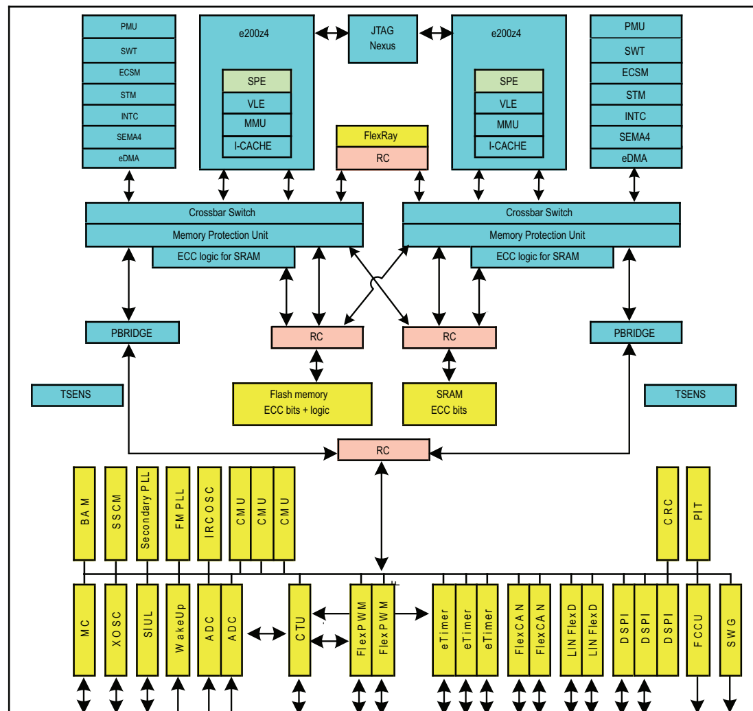
Figure 1. SPC56EL60 block diagram
