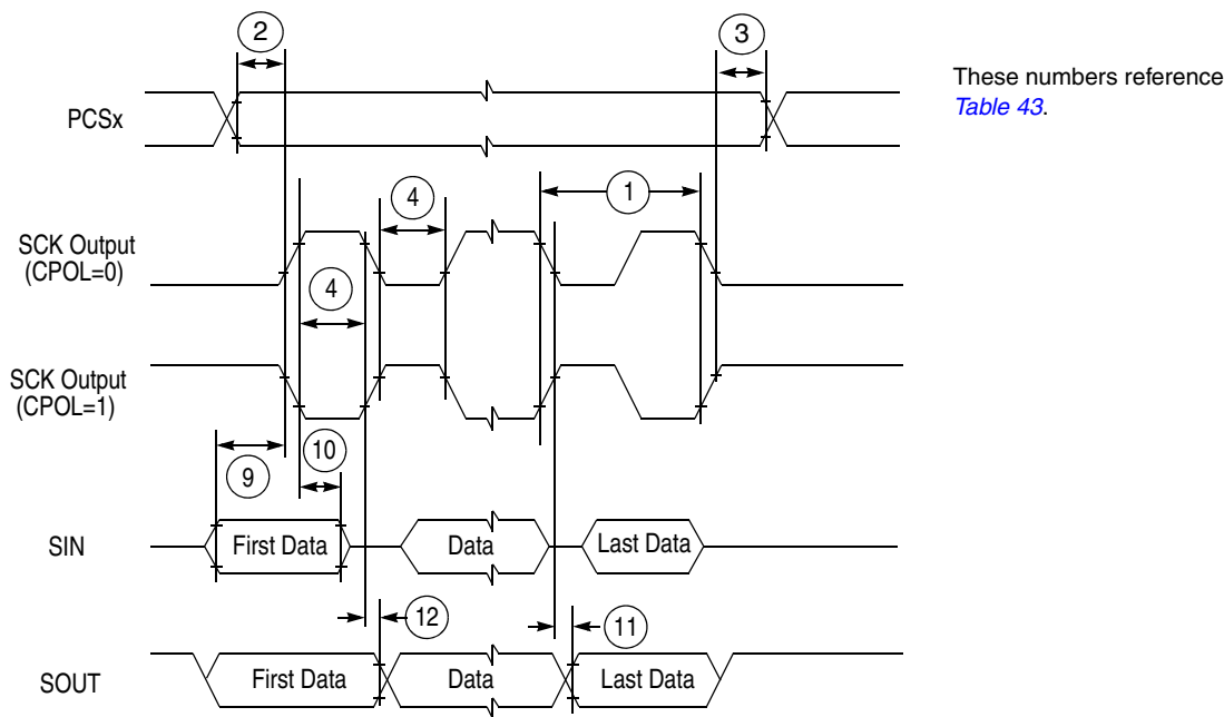
Figure 20. DSPI classic SPI timing – master, CPHA = 0
