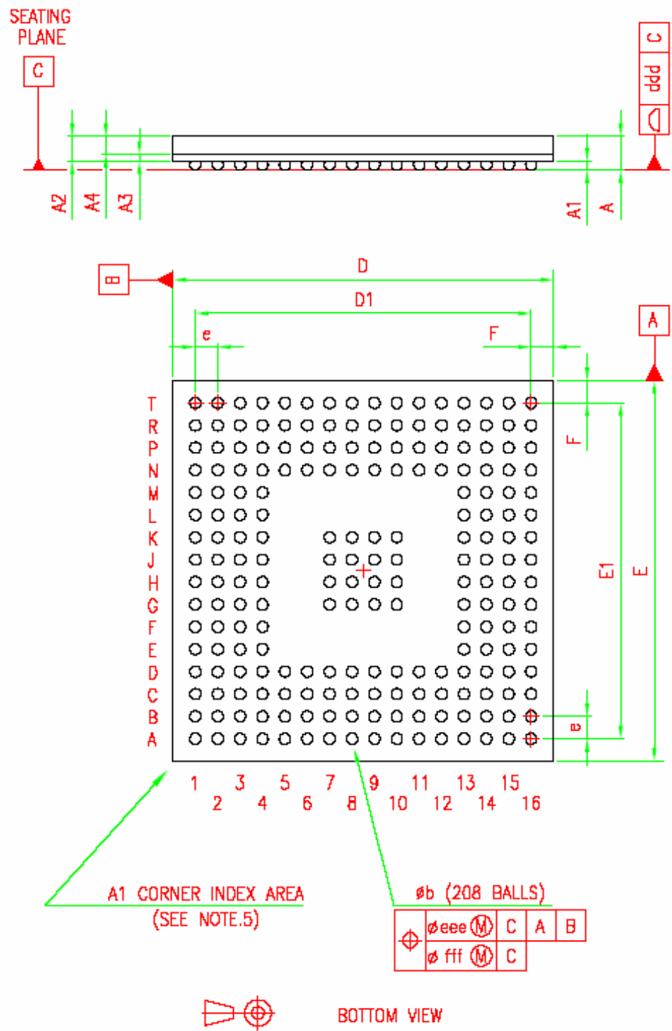
Figure 33. LPGA208 package mechanical drawing
