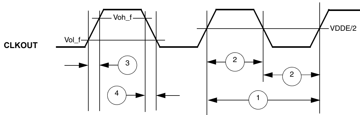
Figure 16. CLKOUT timing
