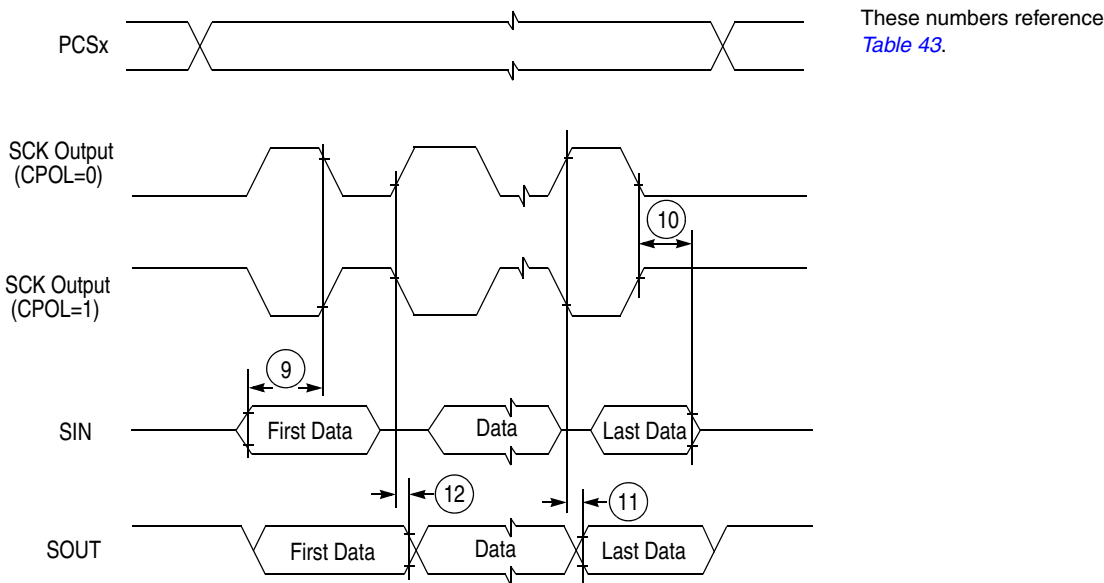
Figure 21. DSPI classic SPI timing – master, CPHA = 1
