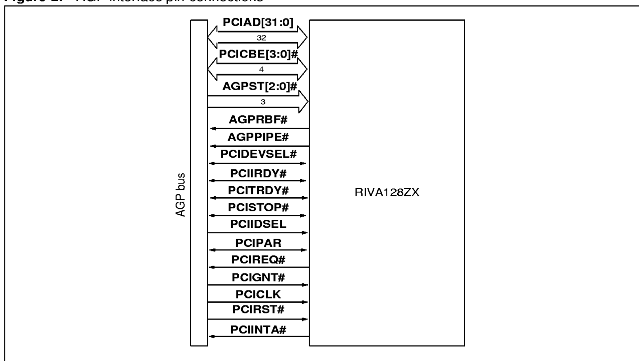
Figure 2. AGP interface pin connections
