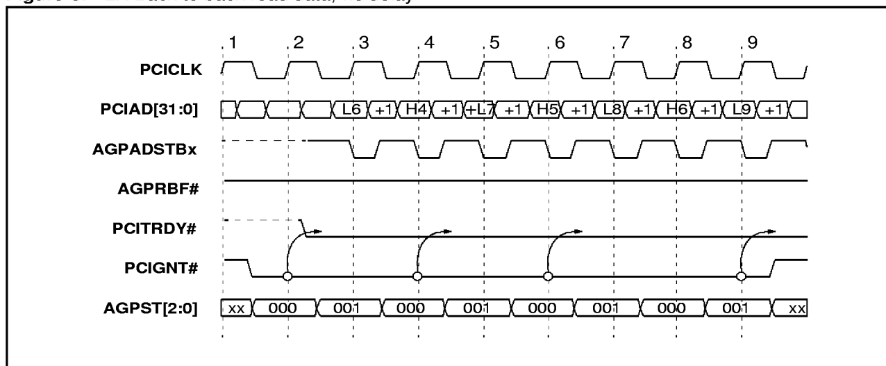
Figure 9. 2X Back to back read data, no delay
