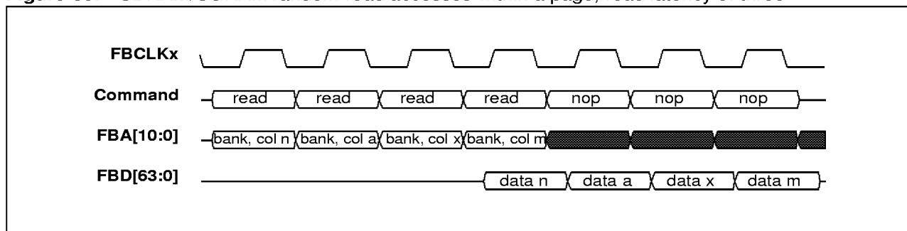
Figure 35. SDRAM/SGRAM random read accesses within a page, read latency of three 1
