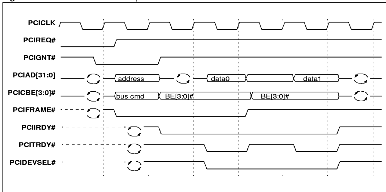
Figure 23. PCI Master read - multiple word
