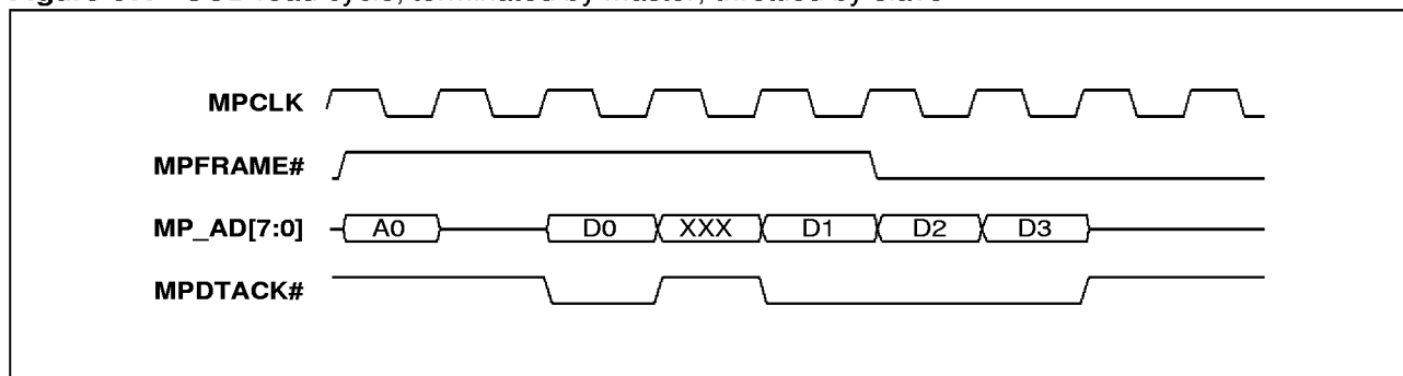
Figure 57. UCD read cycle, terminated by master, throttled by slave
