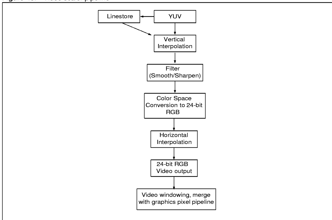
Figure 43. Video scaler pipeline
