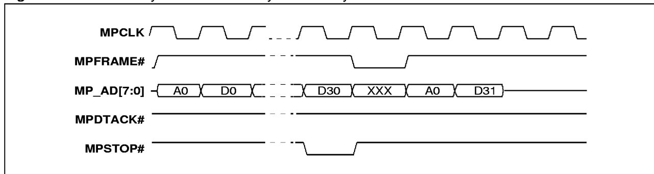
Figure 56. CD write cycle - terminated by slave on byte 32, no effect
