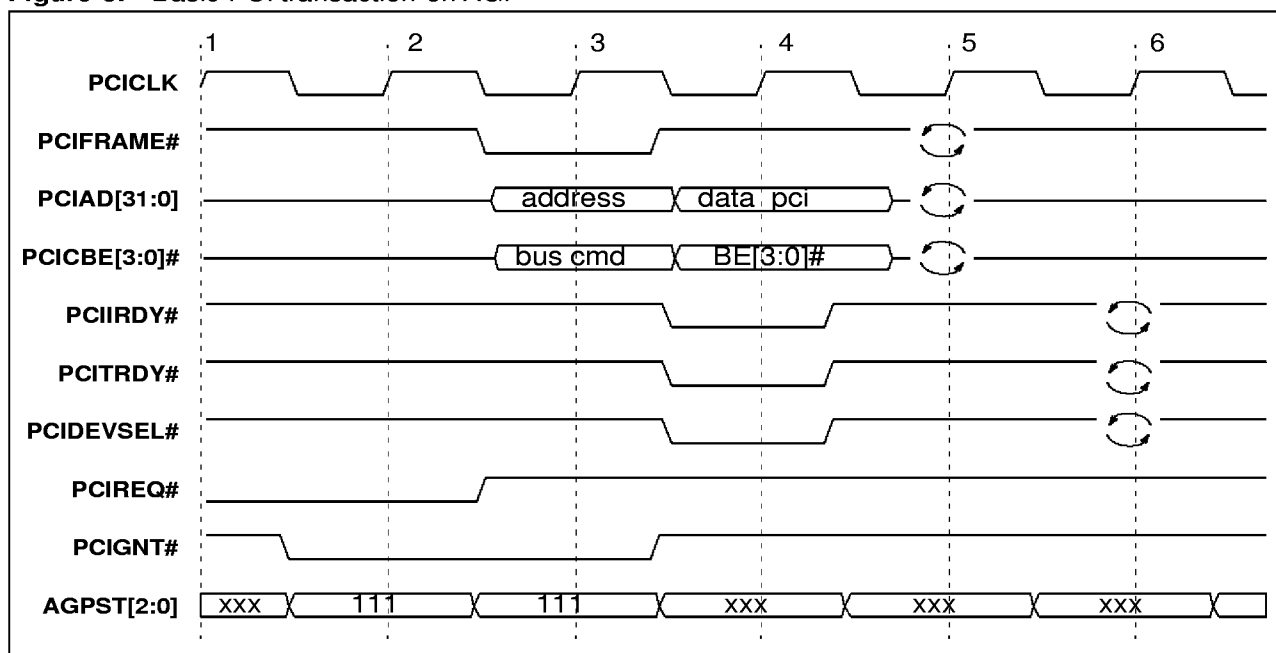
Figure 3. Basic PCI transaction on AGP
