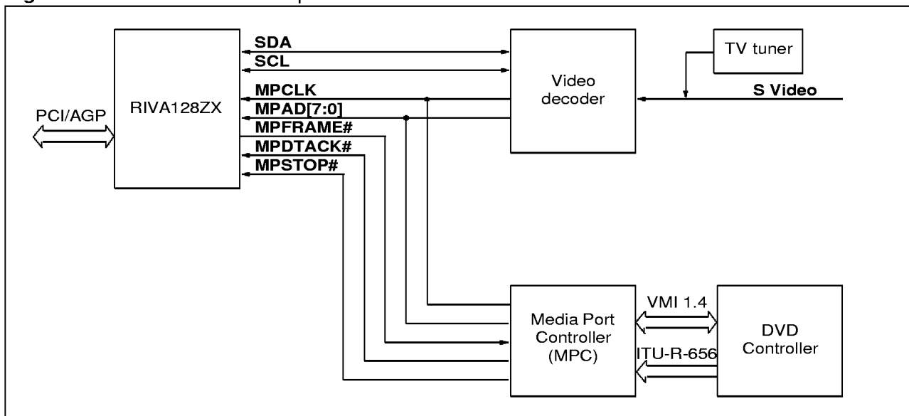
Figure 45. Connections to multiple video modules
