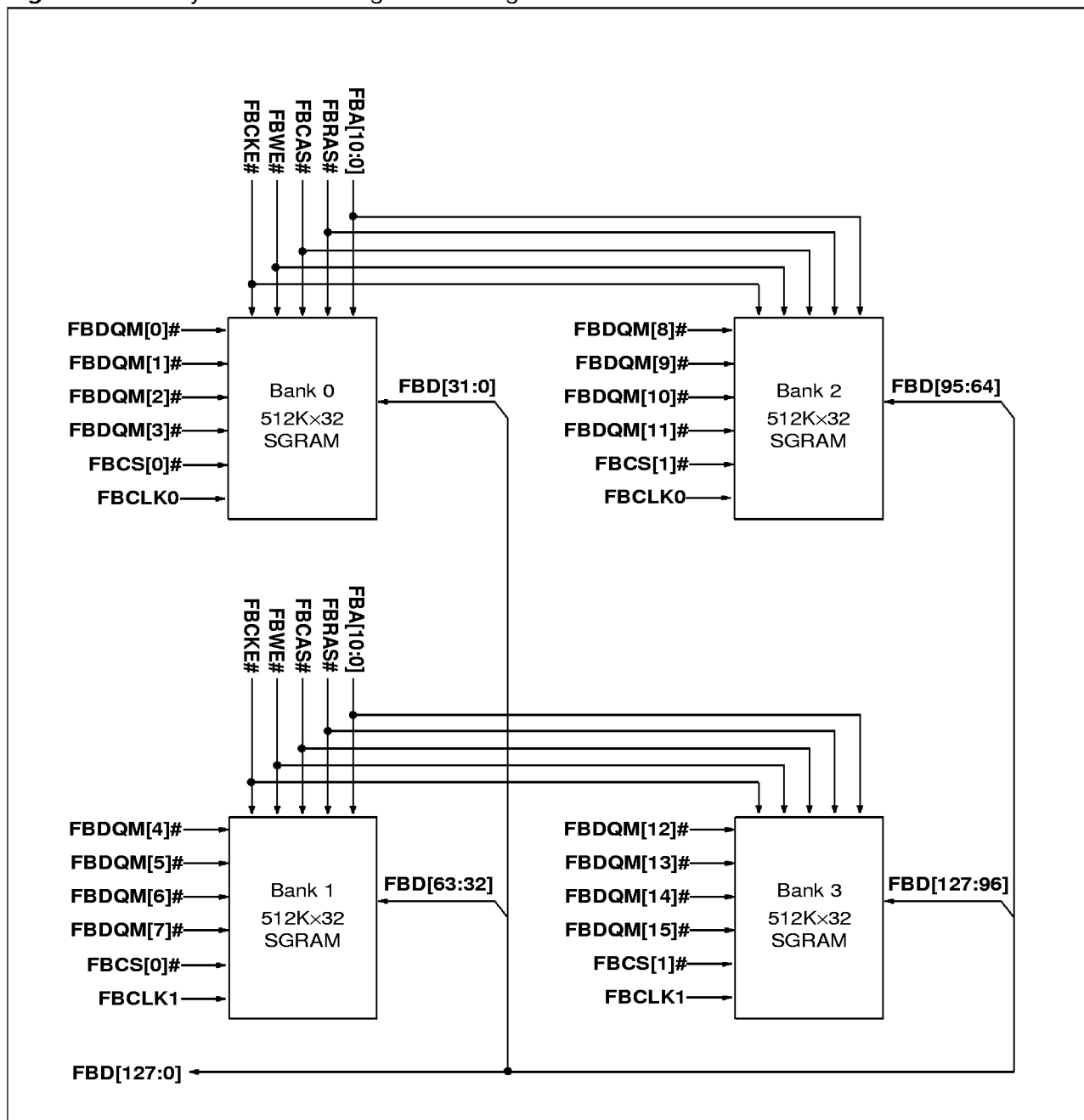
Figure 31. 8MByte SGRAM configuration using 16Mbit devices
