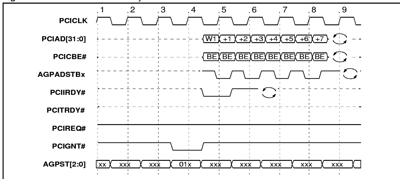
Figure 10. 2X Basic write no delay
