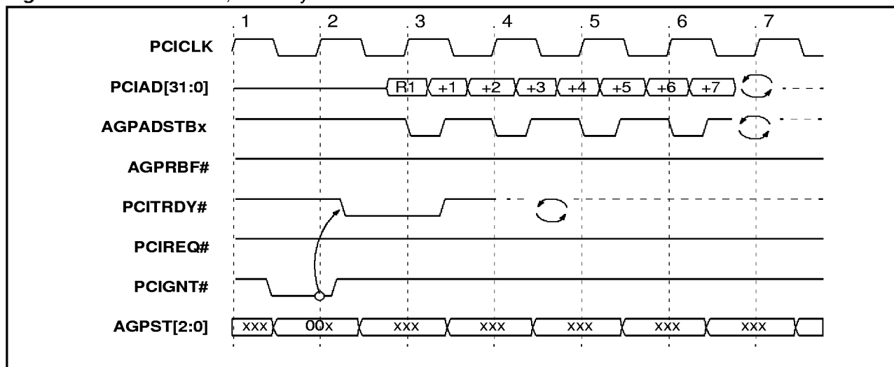
Figure 8. 2X Read data, no delay
