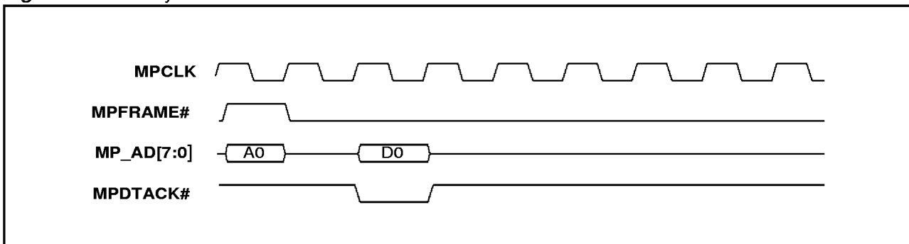
Figure 47. Poll cycle throttled by slave
