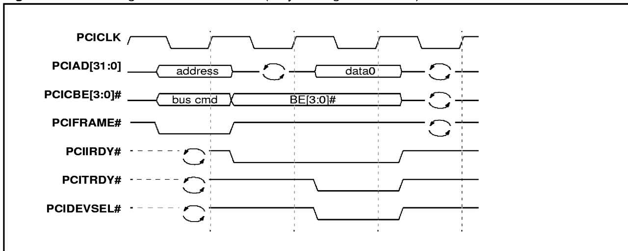
Figure 21. PCI Target read - Slave Read (slow single word read)
