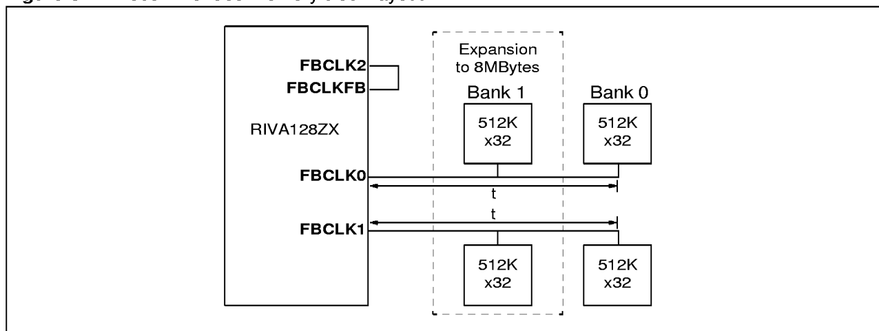
Figure 32. Recommended memory clock layout
