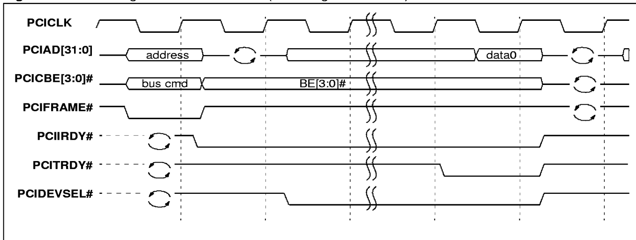
Figure 21. PCI Target read - Slave Read (slow single word read)
