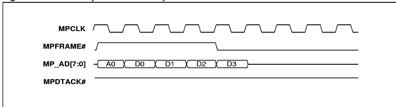
Figure 53. CD write cycle - terminated by master
