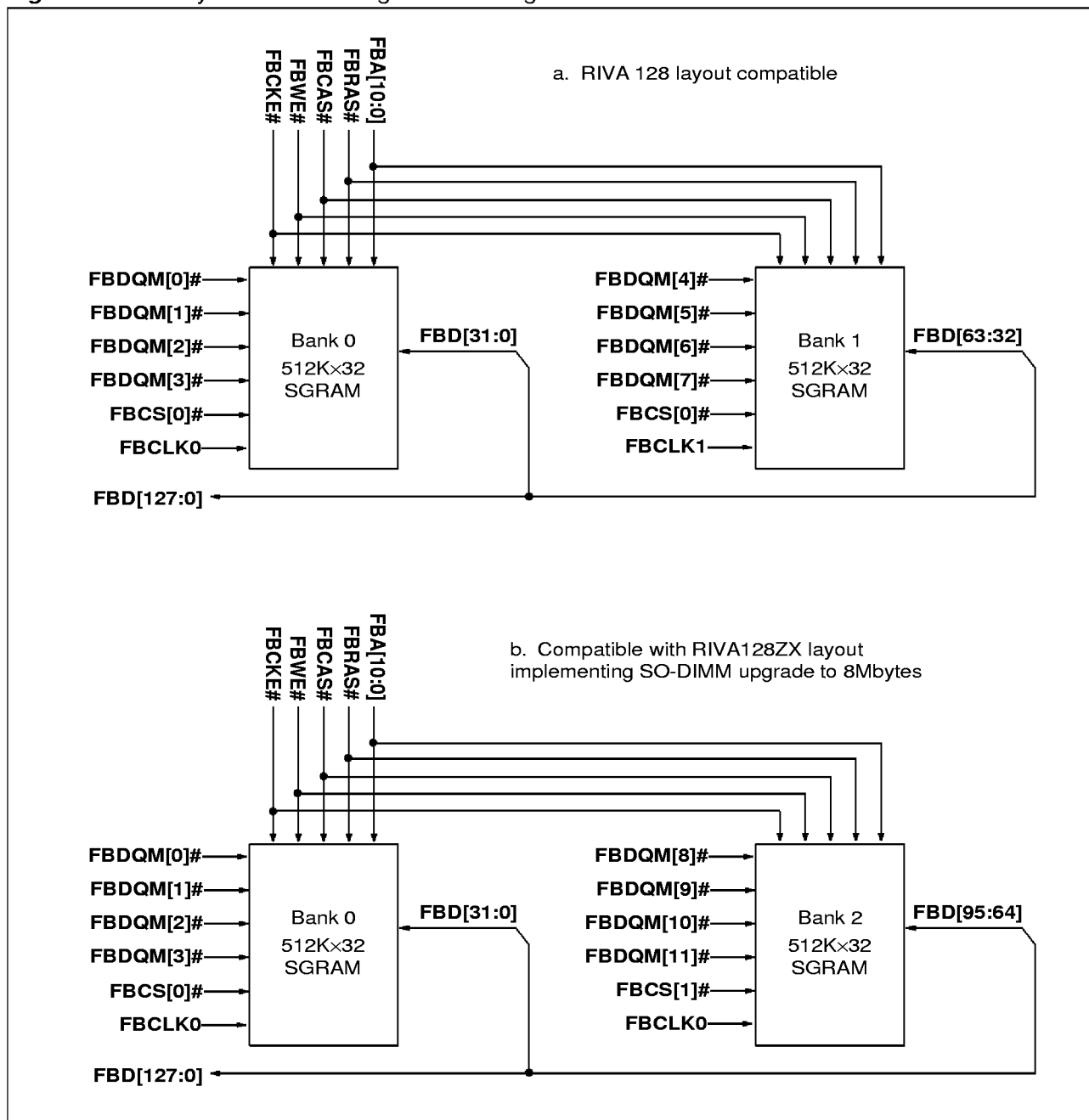
Figure 30. 4 MByte SGRAM configurations using 16Mbit devices
