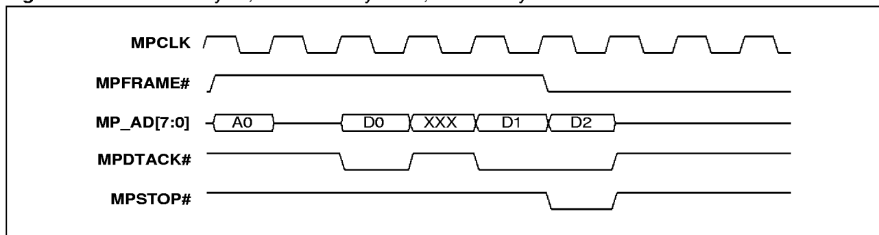
Figure 59. UCD read cycle, slave termination after MPFRAME# deasserted, data taken
