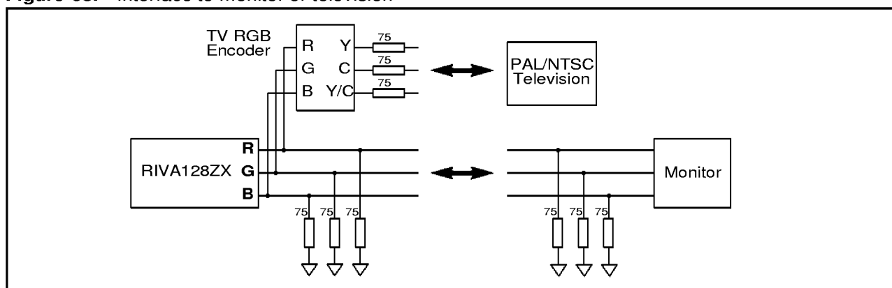
Figure 68. Interface to monitor or television
