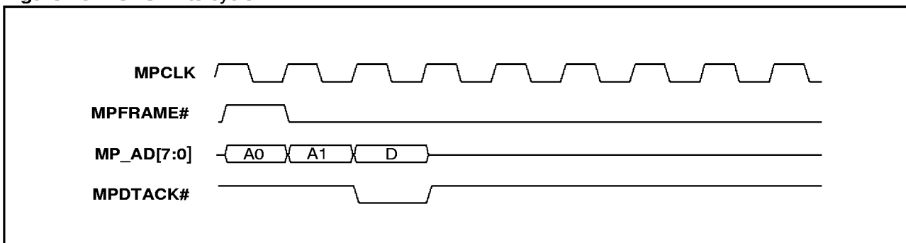
Figure 49. CPU write cycle throttled by slave
