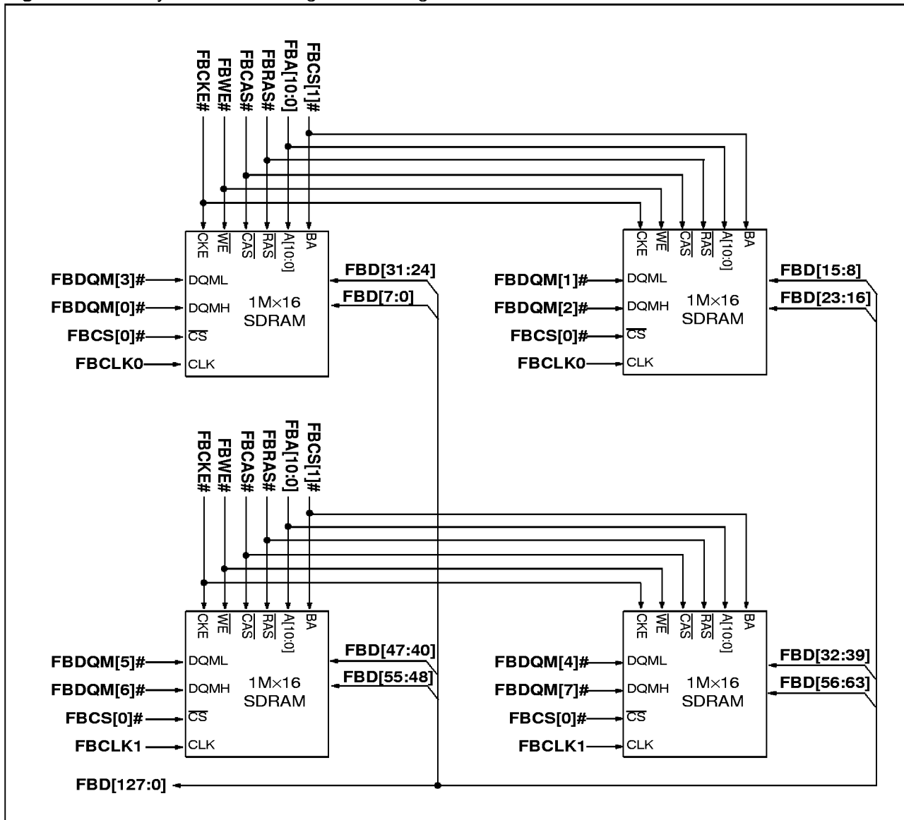
Figure 28. 8MByte SDRAM configuration using 16Mbit devices
