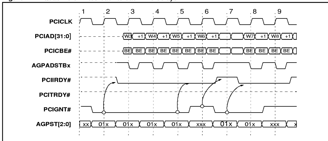
Figure 11. QuadWord writes back to back - no delays
