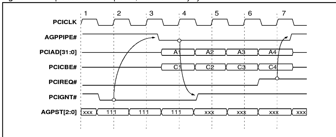
Figure 7. Multiple addresses enqueue, maximum delay by RIVA128ZX
