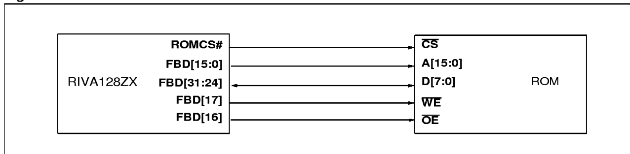
Figure 63. ROM interface
