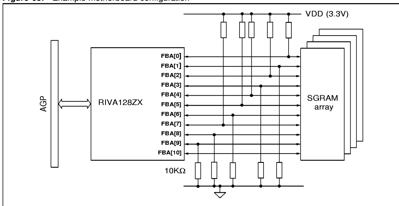
Figure 65. Example motherboard configuration
