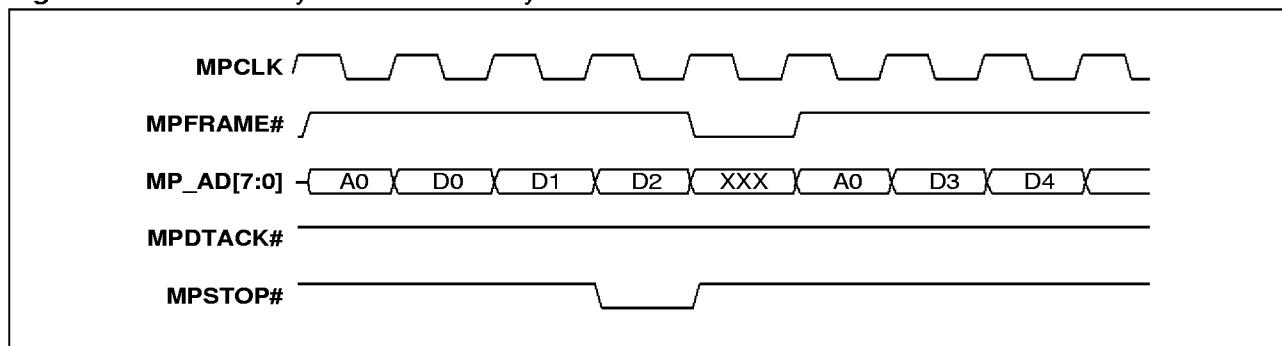
Figure 55. CD write cycle - terminated by slave on byte 31
