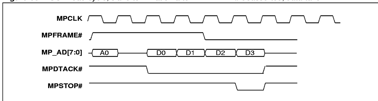
Figure 60. UCD read cycle, slave termination after MPFRAME# deasserted, data not taken
