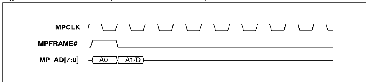
Figure 51. CPU read_receive cycle
