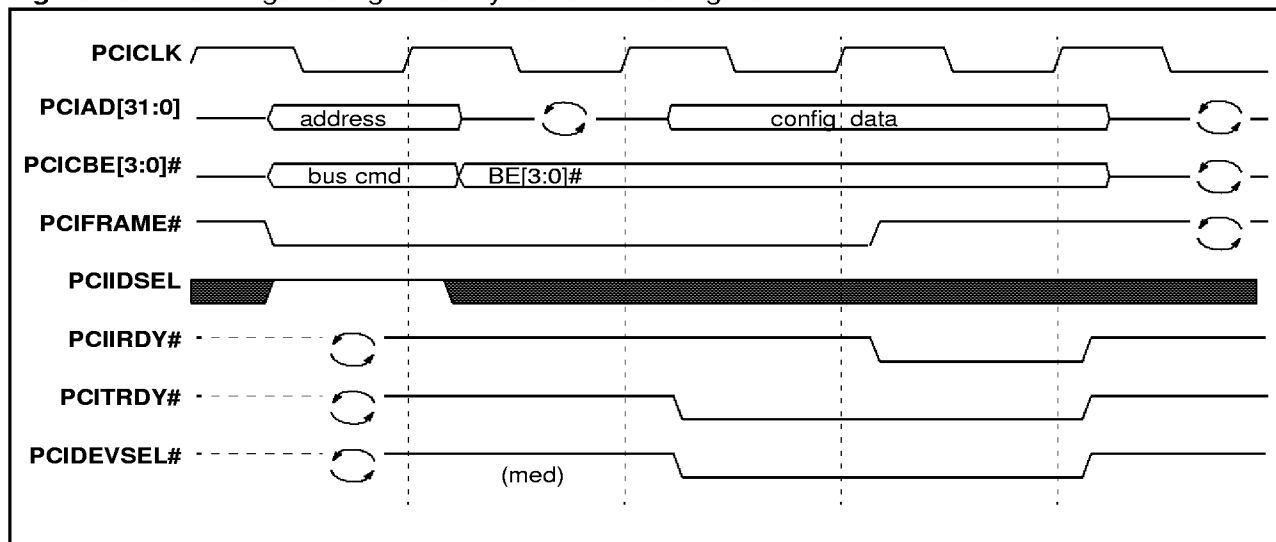
Figure 25. PCI Target configuration cycle - Slave Configuration Read
