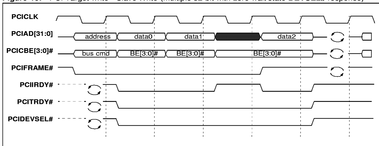
Figure 19. PCI Target write - Slave Write (multiple 32-bit with zero wait state DEVSEL# response)
