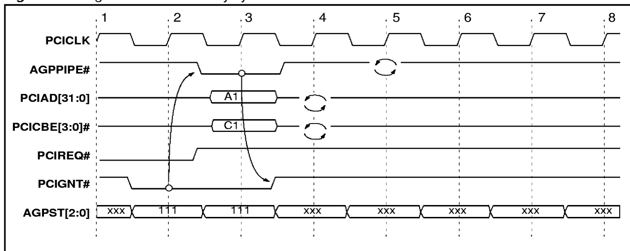
Figure 6. Single address - no delay by master
