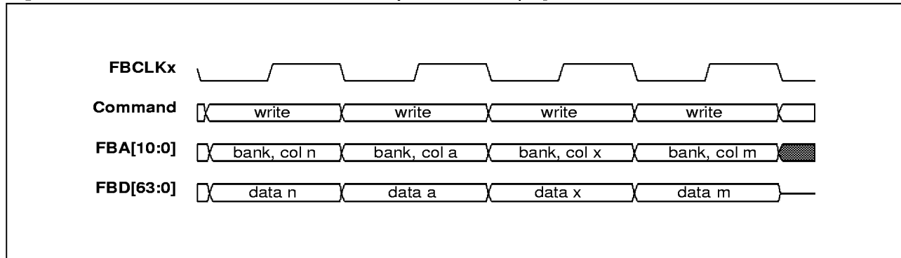
Figure 37. SDRAM/SGRAM random write cycles within a page
