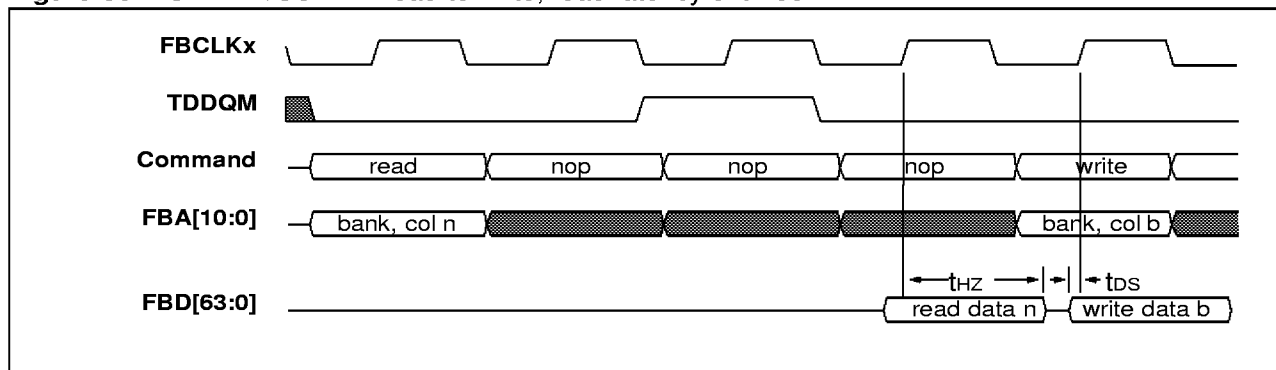
Figure 36. SDRAM/SGRAM read to write, read latency of three
