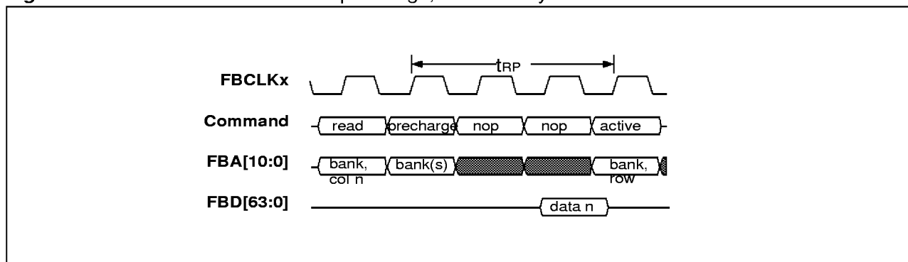
Figure 40. SDRAM/SGRAM read to precharge, read latency of three
