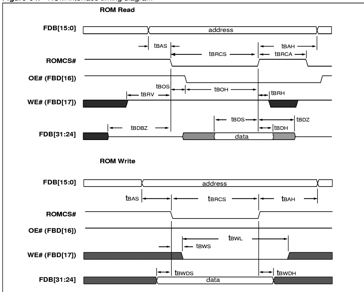
Figure 64. ROM interface timing diagram
