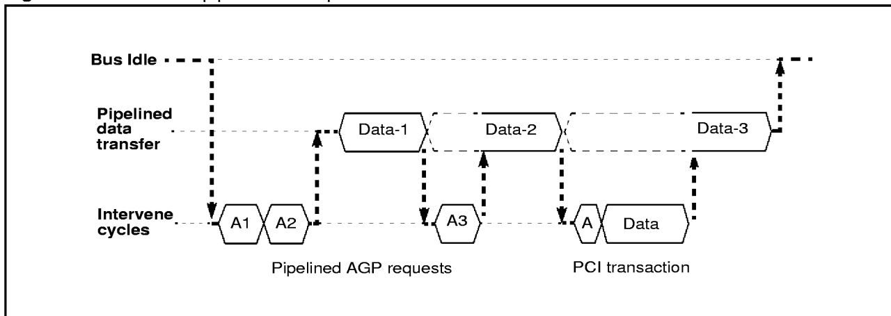
Figure 5. Basic AGP pipeline concept
