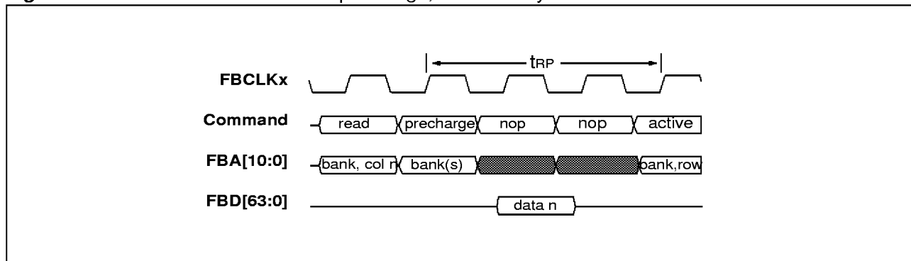
Figure 39. SDRAM/SGRAM read to precharge, read latency of two
