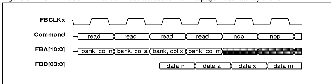
Figure 34. SDRAM/SGRAM random read accesses within a page, read latency of two 1
