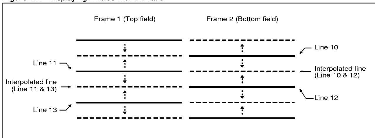
Figure 44. Displaying 2 fields with 1:1 ratio
