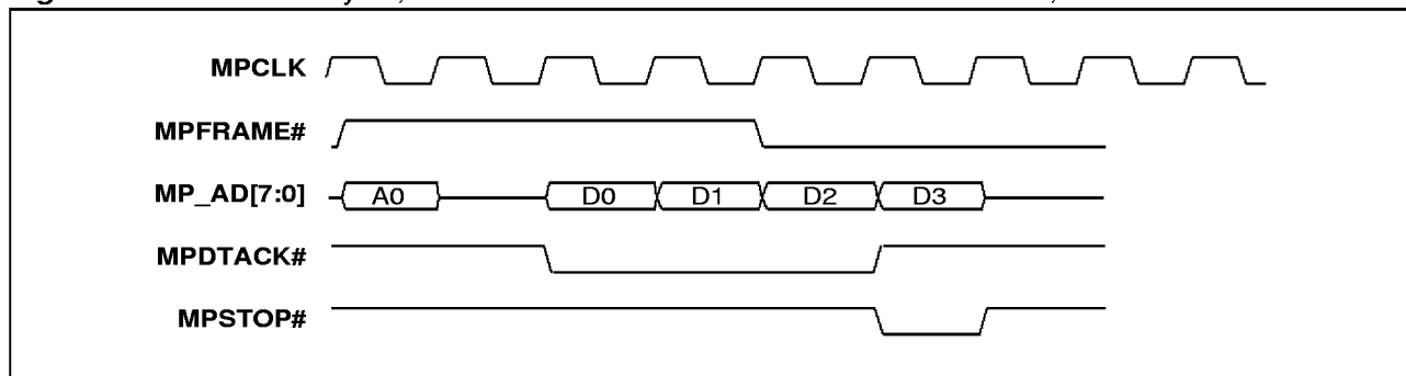
Figure 61. UCD read cycle, slave termination after MPFRAME# deasserted, data taken
