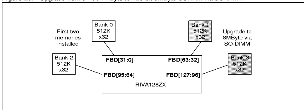
Figure 29. Upgrade from 64-bit 4MByte to 128-bit 8MByte SGRAM via SO-DIMM
