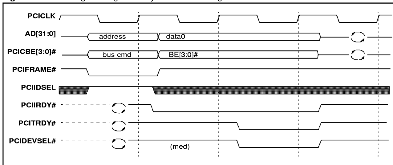
Figure 25. PCI Target configuration cycle - Slave Configuration Read
