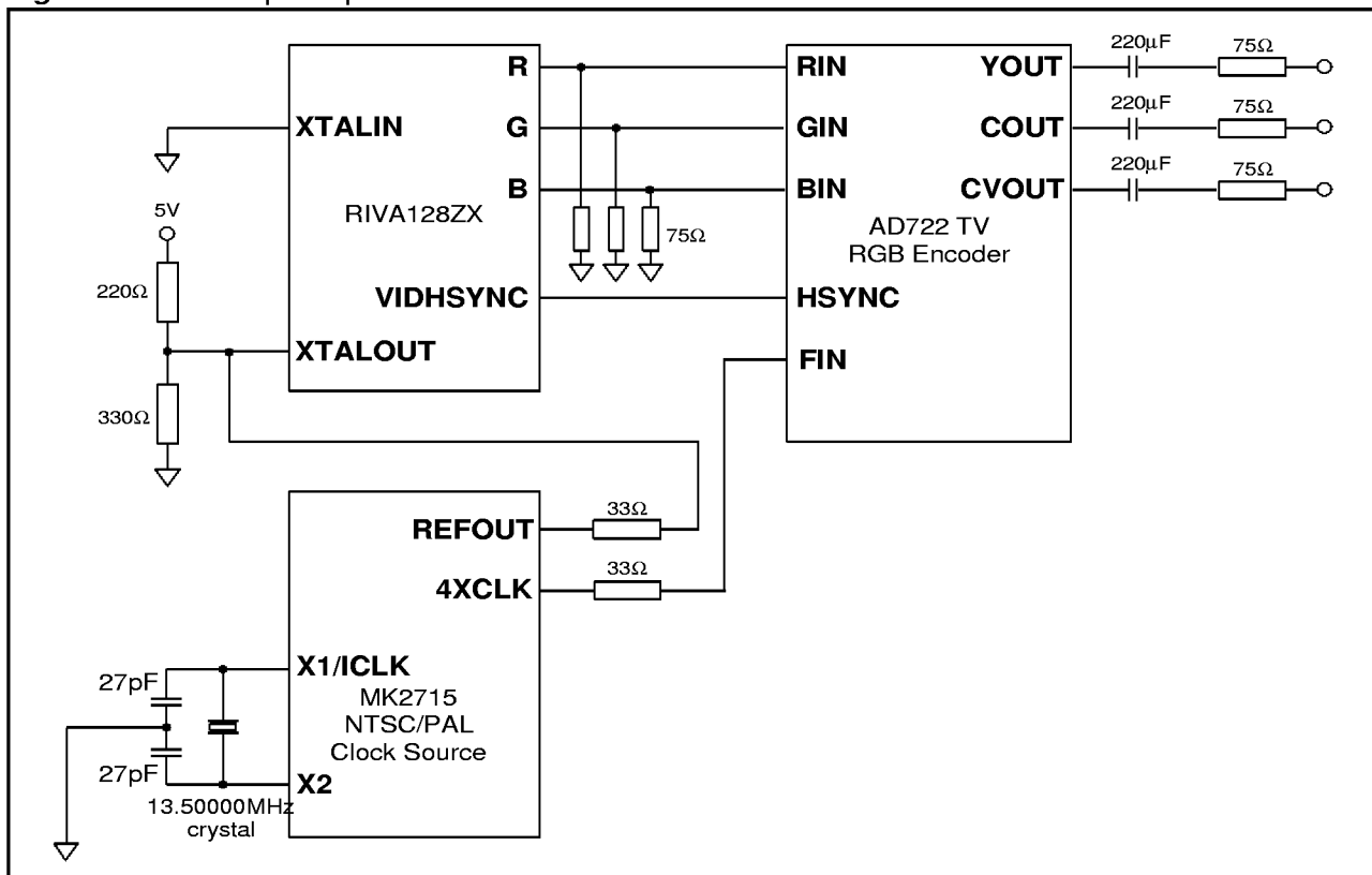
Figure 67. TV output implementation
