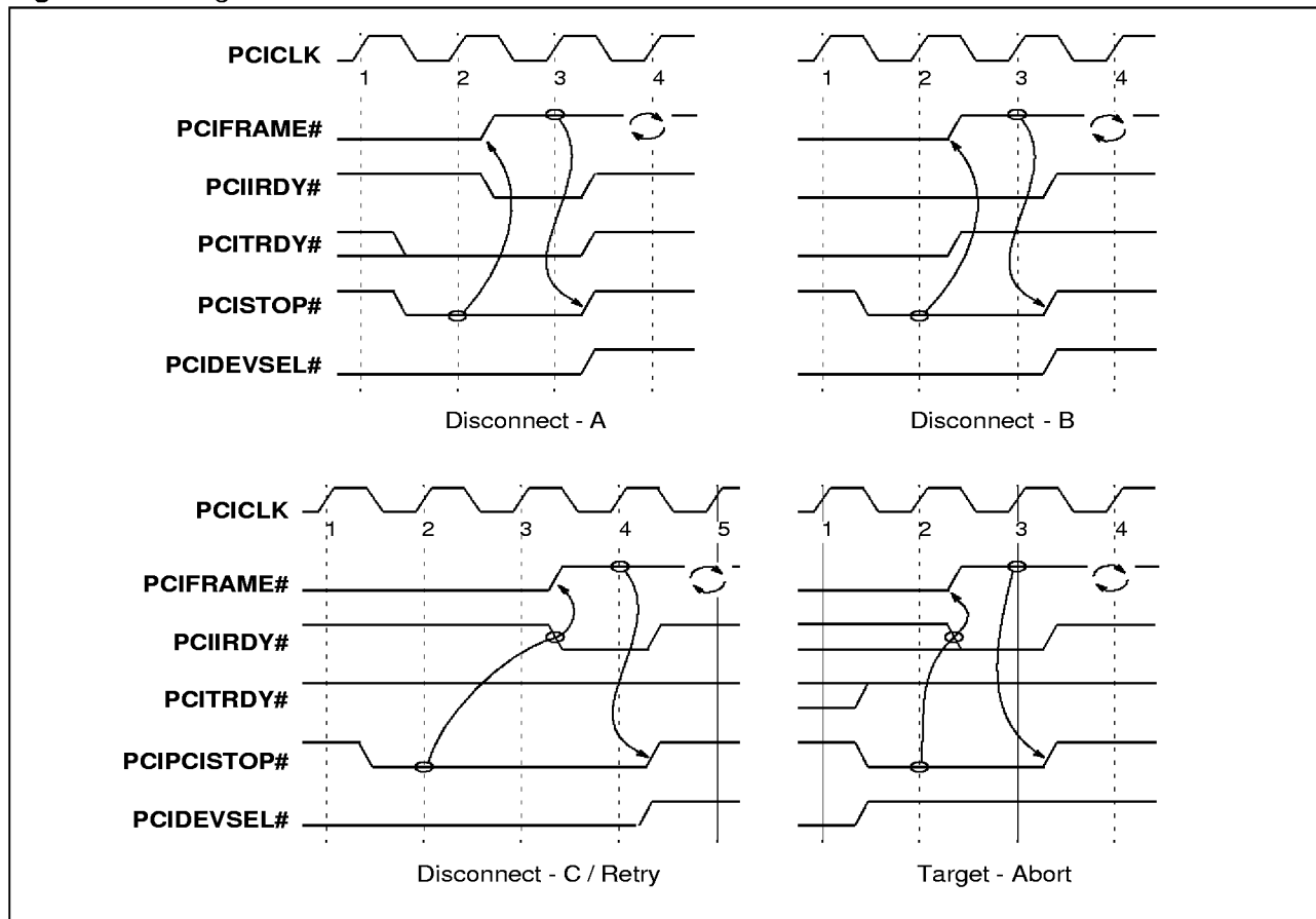
Figure 27. Target initiated termination
