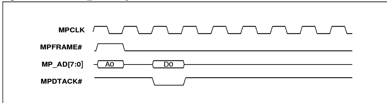
Figure 52. CPU read_receive cycle - throttled by slave
