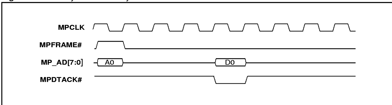
Figure 48. CPU write cycle
