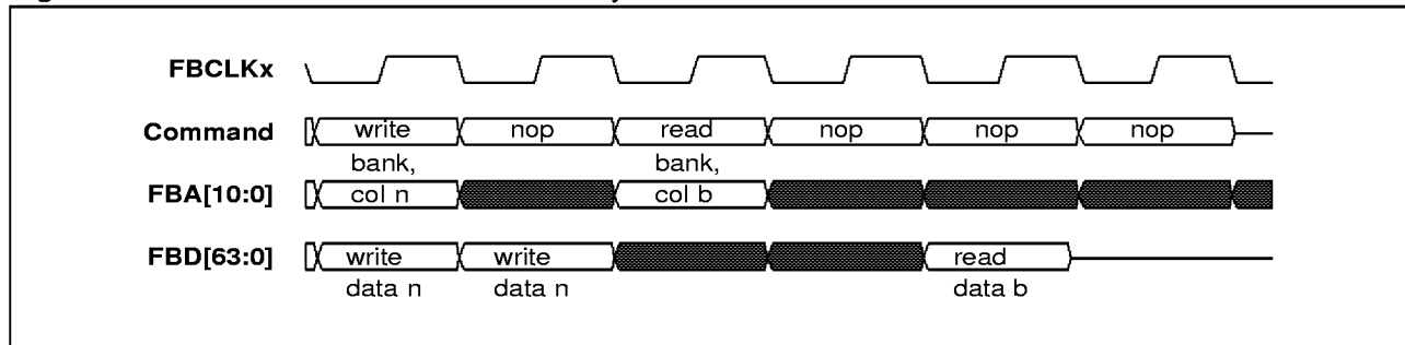
Figure 38. SDRAM/SGRAM write to read cycle
