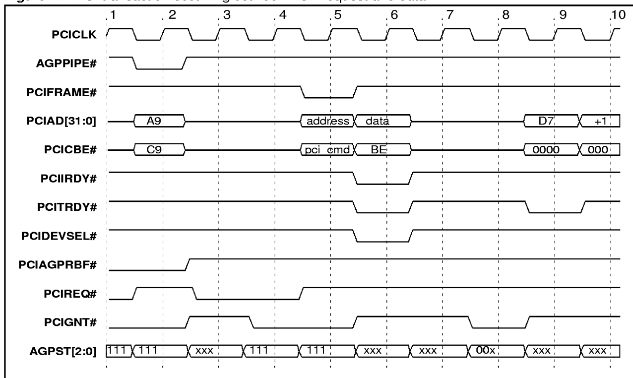
Figure 4. PCI transaction occurring between AGP request and data
