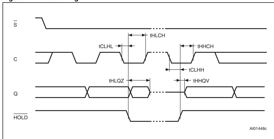
Figure 17. Hold timing
