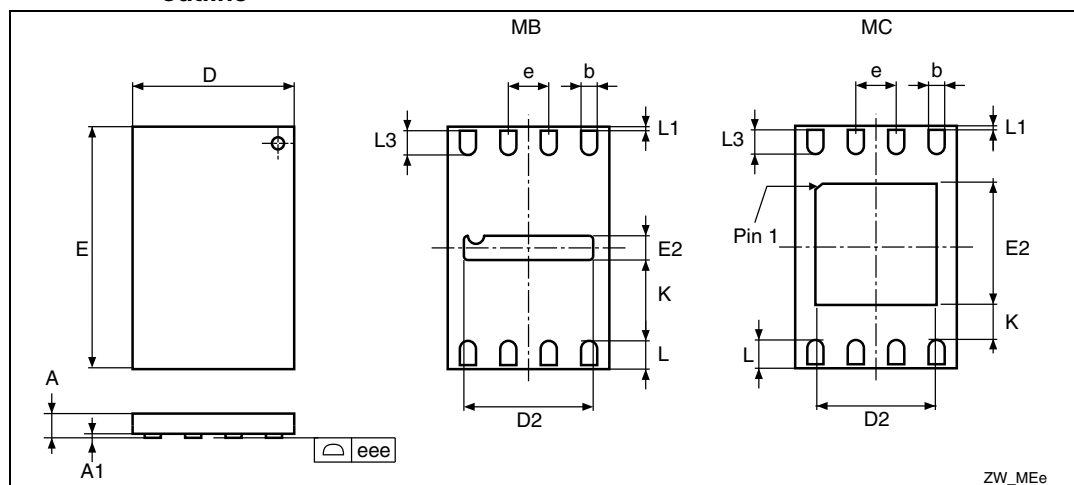
Figure 20. UDFPN8 (MLP8) - 8-lead ultra thin fine pitch dual flat no lead, package outline
