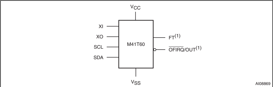
Figure 1. Logic diagram
