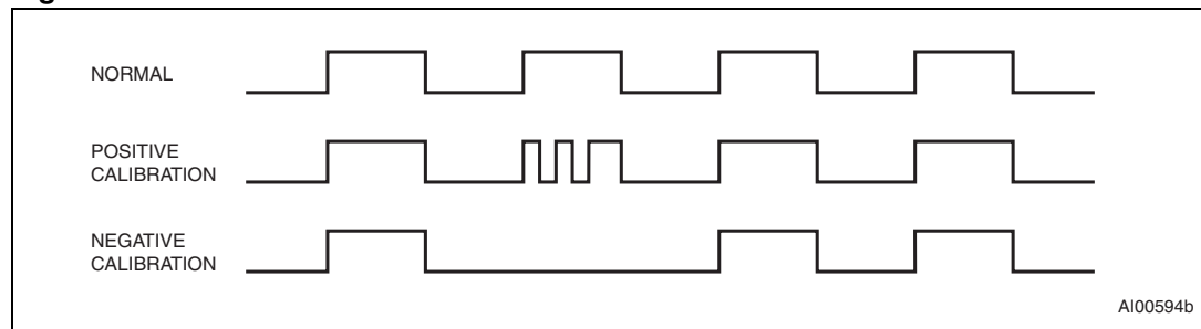
Figure 12. Calibration waveform
