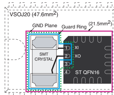
Footprint comparison of ST's QFN16 with SMT crystal vs. competing VSOJ20 package
