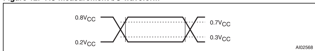
Figure 12. AC measurement I/O waveform
