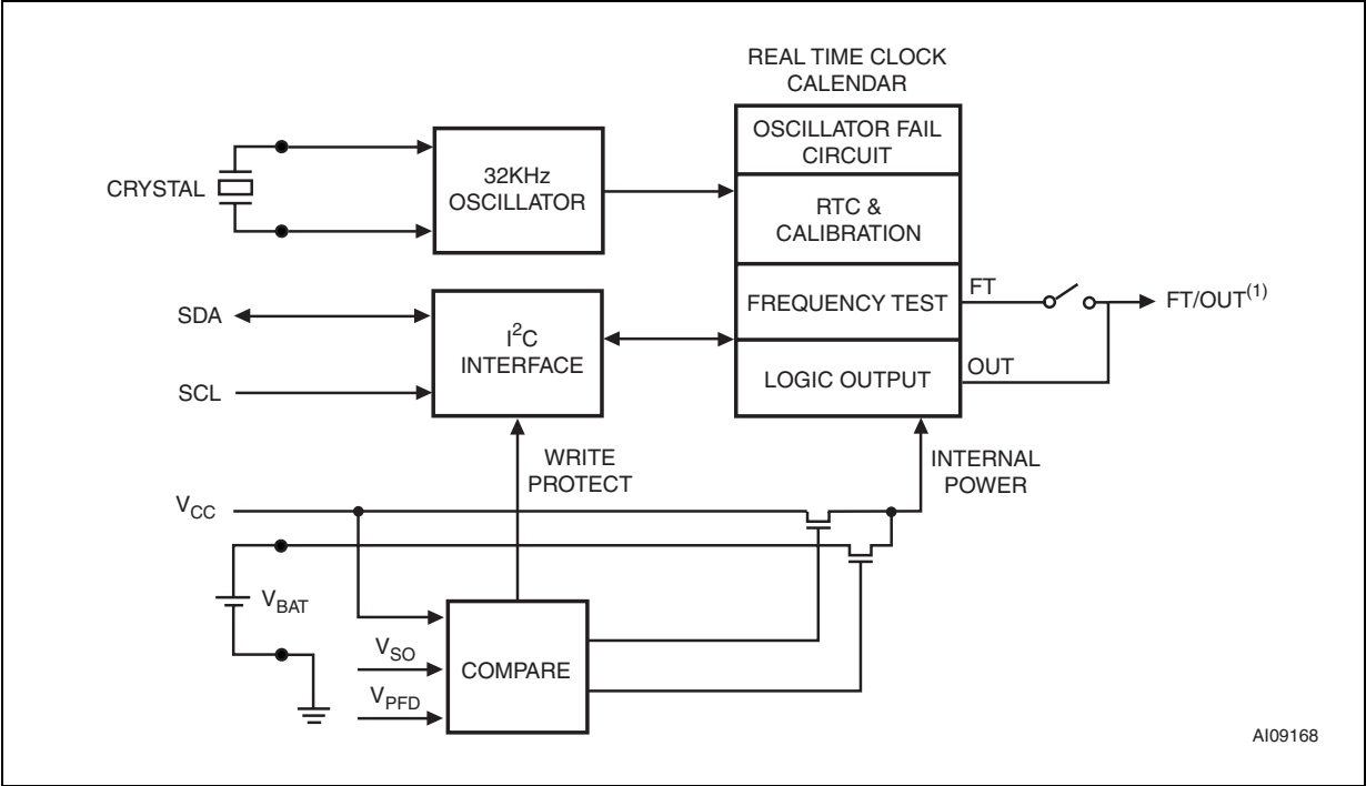
Figure 3. Block diagram
