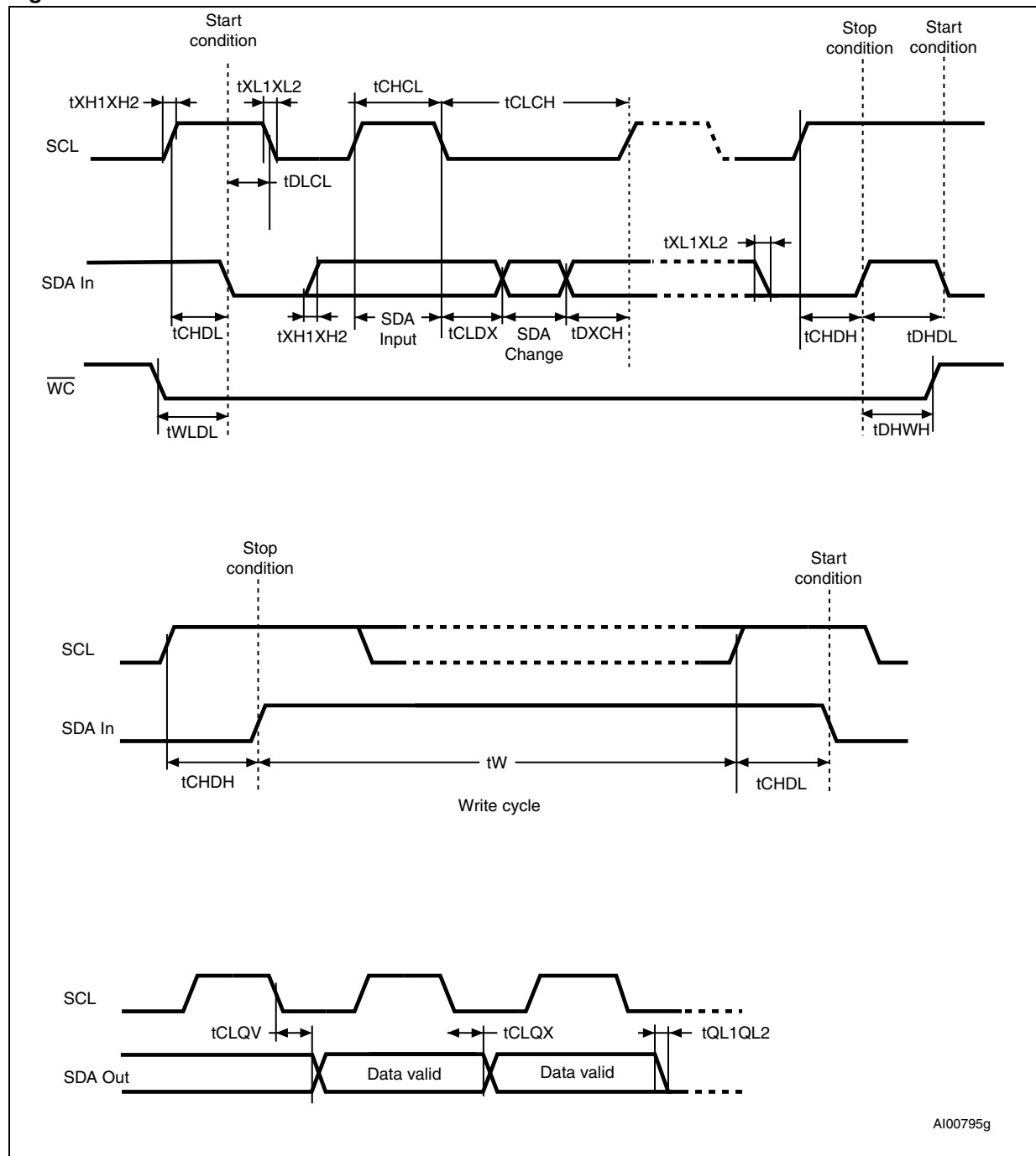
Figure 12. AC waveforms
