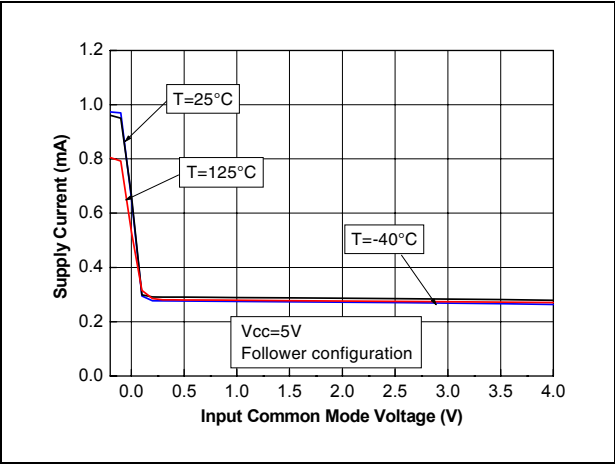
Figure 3. Supply current vs. input common mode voltage in a follower configuration at V_{CC} = 5\text{ V}
