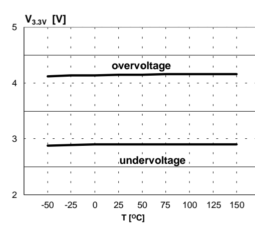
Figure 6. 3.3V fault thresholds
