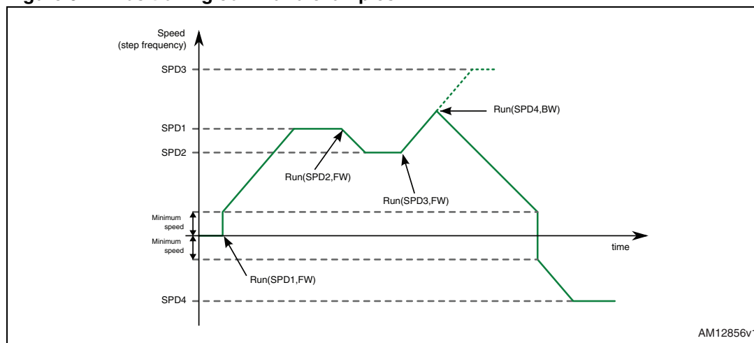
Figure 9. Positioning command examples
