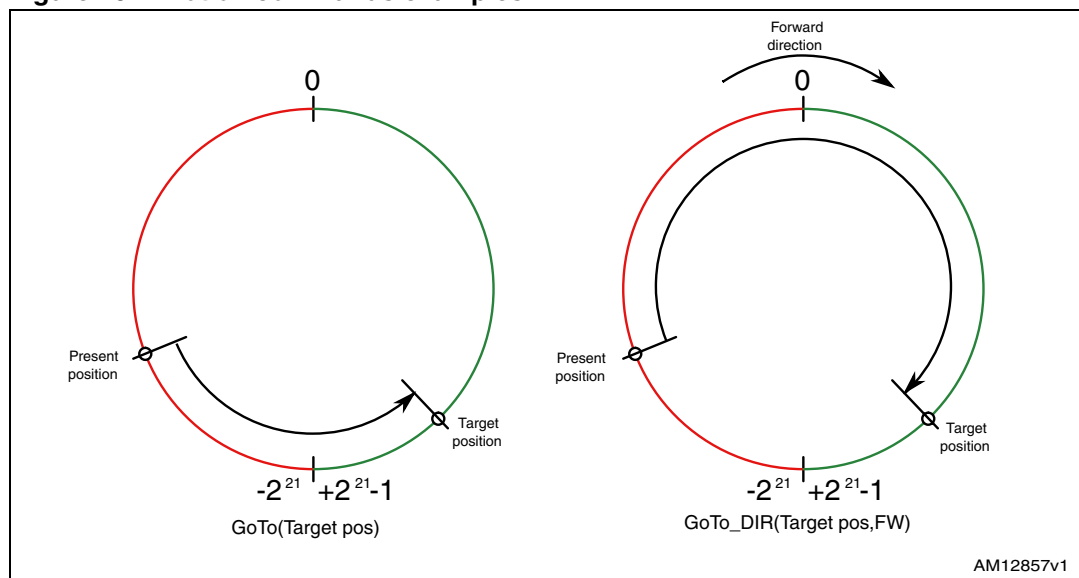
Figure 10. Motion commands examples
