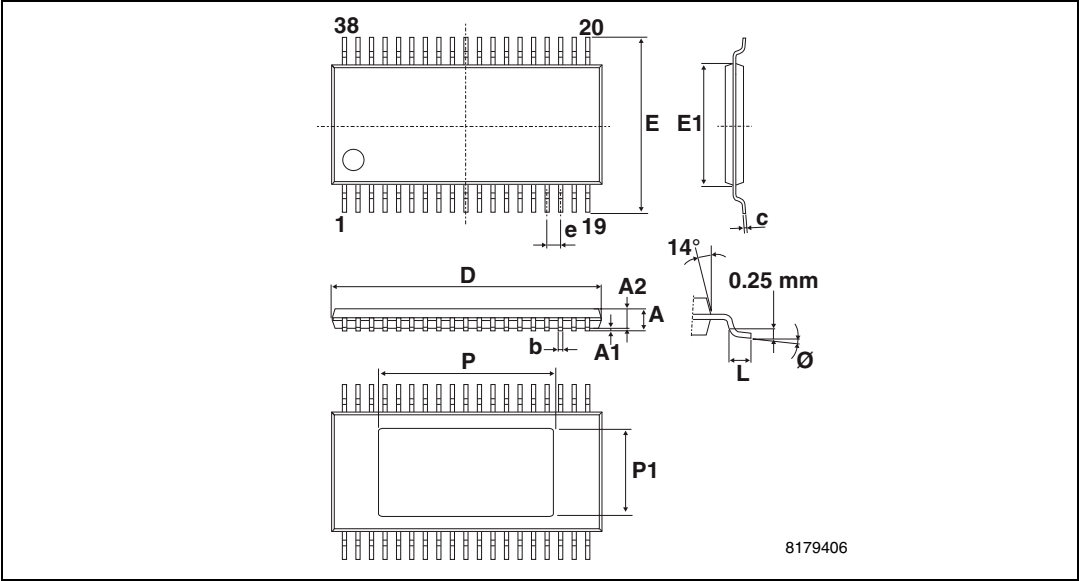
Figure 24. HTSSOP38 package dimensions
