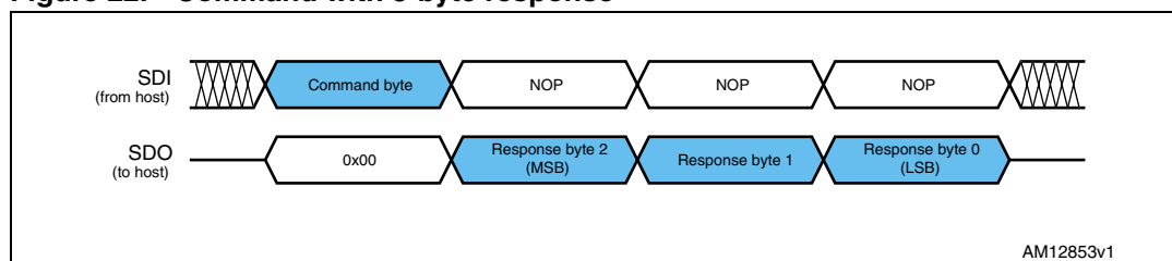
Figure 22. Command with 3-byte response
