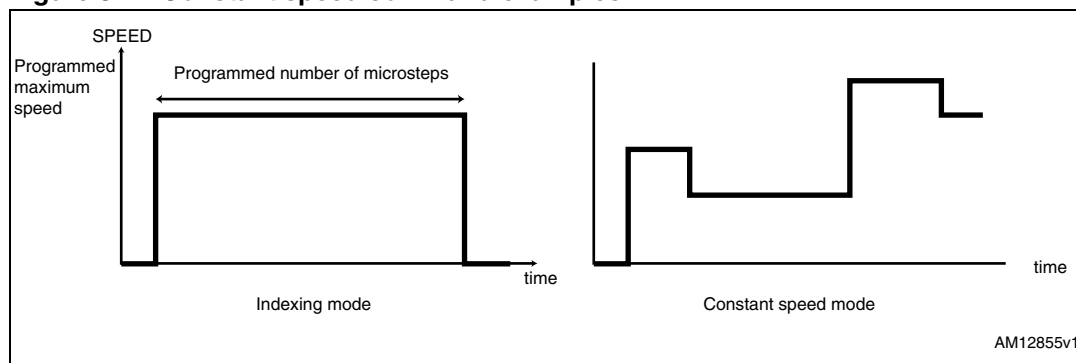
Figure 8. Constant speed command examples
