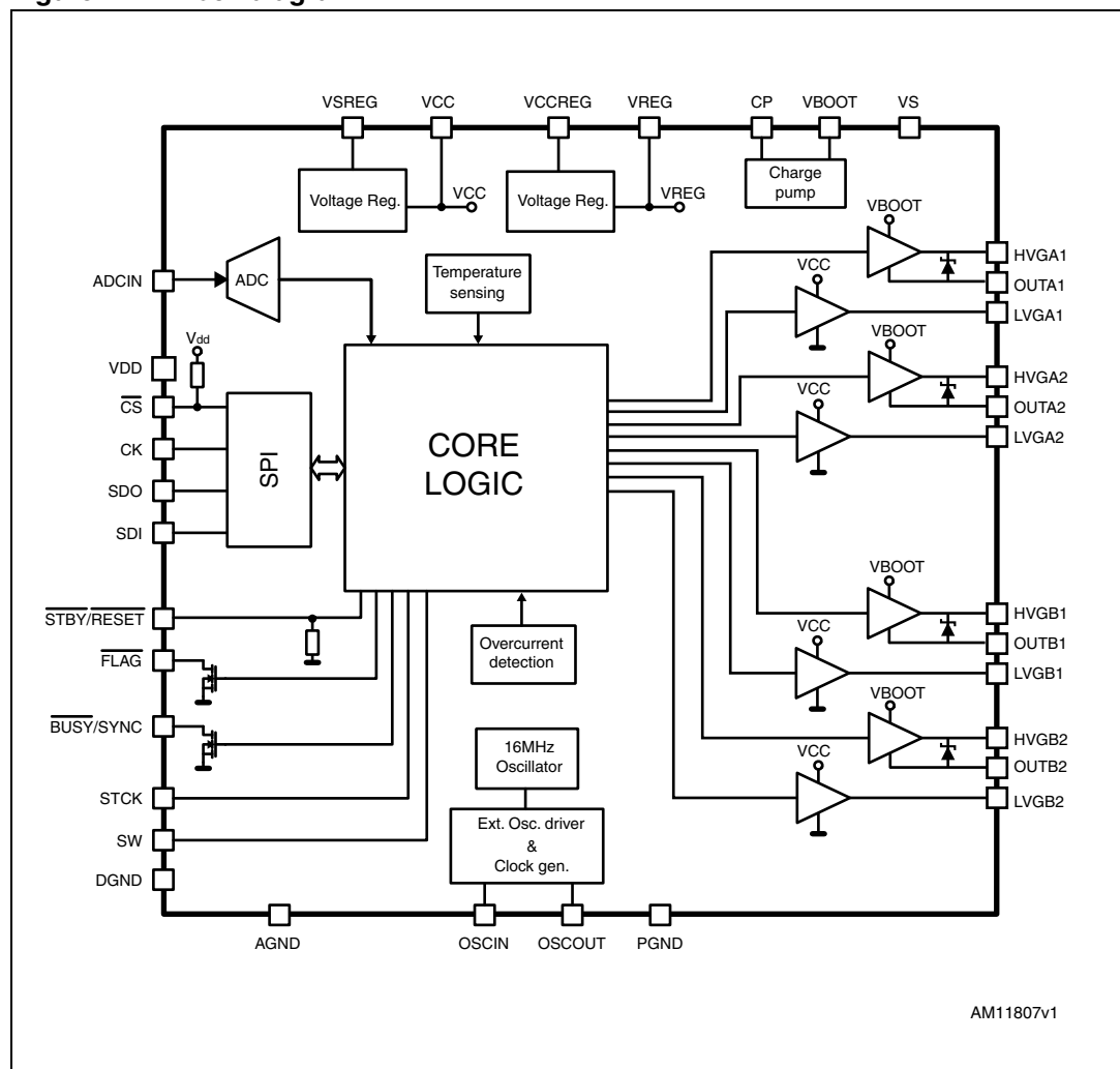
Figure 1. Block diagram
